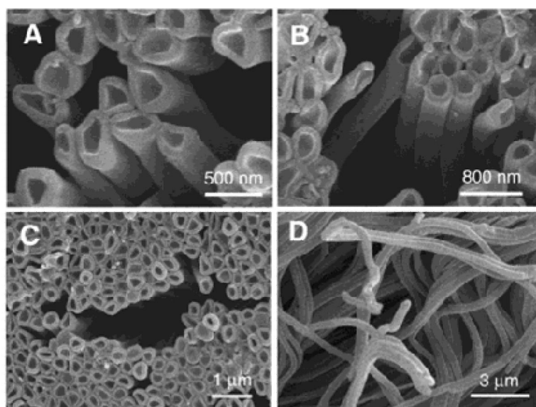
FIGURE 2. Scanning electron micrographs at different magnifications (A-D) of polyelectrolyte nanotubes obtained via nanotemplated LbL assembly of poly(allylamine) and poly(styrene sulfonate). Reproduced with permission from Ai et al. J. Am. Chem. Soc. , 2003, 125 , 11140. Copyright 2003 American Chemical Society.
