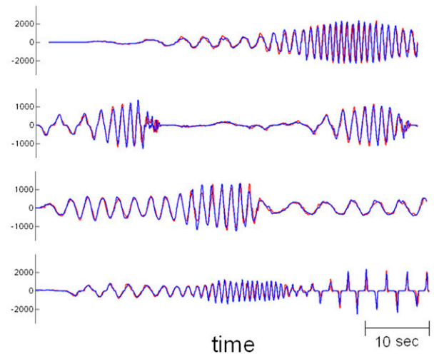
Fig. 1. A one-dimensional mirror game shows complex, coordinated improvised motion. (A) In the mirror game, the motion of two players moving handles along tracks is sampled at 50 Hz and at a spatial resolution of 0.94 mm. (B) Examples of velocity traces in rounds where the leader and follower are designated (LF rounds). Here the leader is the blue player. (C) Examples of velocity traces in joint improvisation rounds, with no designated leader and follower (JI rounds). The data for all experimental rounds are provided in SI Appendix, Fig. 24 .
