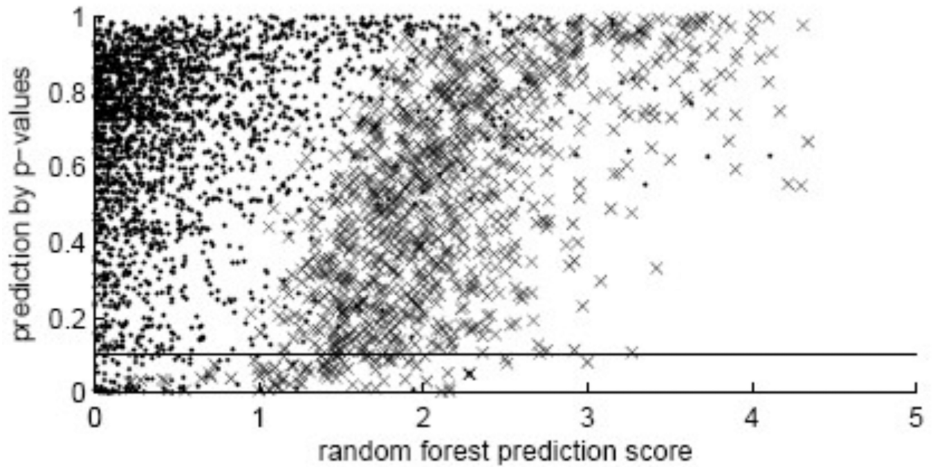
Fig. 1. Random Forest (RF) prediction scores 6 (where they are positive) and p-values obtained by the conformal predictor for the same pairs. Crosses (interactions) are known interactions, other examples are represented as points. Examples with RF prediction score less than zero are not included. The horizontal line corresponds to 10% cut-off for p-value (significance level), or confidence level 90% (for a true interaction, we are 90% sure that it is above this line).
