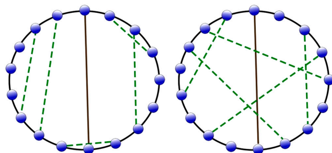
Fig. 7. The left box is a sketch of a typical contact map for the same number of contacts for random distribution of contacts and the right box, for our simulation of interacting nucleosomes. The solid line is the insulator contact (permanent) and dashed lines represent transient contacts between nucleosomes.
