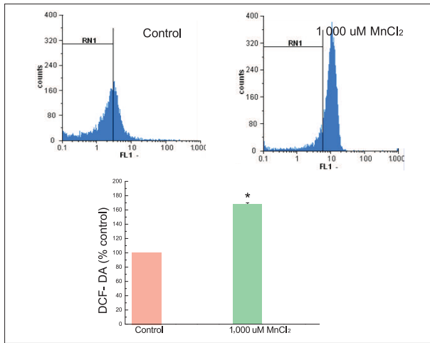
Figure 5. Intracellular ROS induced MnCl 2 . Cells were treated with 1,000 \mu M MnCl 2 and were incubated with dichlorofluorescein diacetate (100 \mu M), then the fluorescence intensities of 10,000 cells were analyzed by flow cytometry (Partec PAS). The DCFDA fluorescence was quantified.
