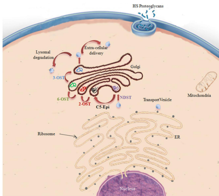
Figure 5. Biosynthesis of HS and heparin in eukaryotic cells. Arrows in red indicate next step within the biosynthetic pathway. C5-Epi: C5-Epimerase, NDST: N -deacetylase/ N -sulfotranferase, 2,3,6-OST: 2,3,6- O -sulfo transferase are the enzymes involved in heparin/HS biosynthetic pathway.
