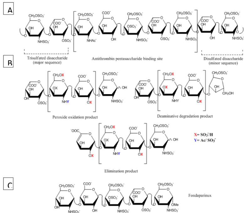
Figure 1. Structure of heparin, LMWH and ULMWH fondaparinux. (A) A representative sequence of heparin comprising a major trisulfated disaccharide sequence, an AT-binding site and a minor disulfated disaccharide sequence (B) LMWH structures generated through peroxide oxidation, deaminative degradation and chemical or enzymatic β-elimination (C) ULMWH, a commercial synthetic pentasaccharide AT-binding domain stabilized as the methyl glycoside called 'fondaparinux'
