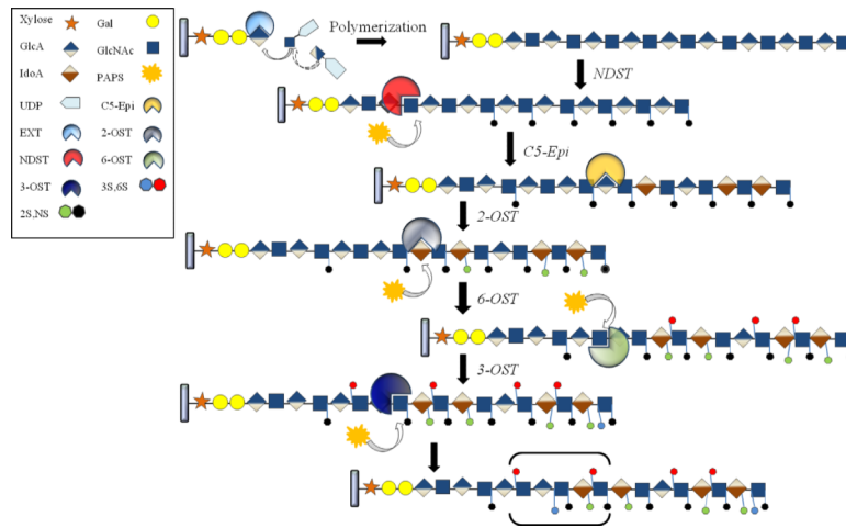
Figure 4. Biosynthetic pathway for heparin and HS. Synthesis of tetrasaccharide linker attached to serine residue of core protein takes place in the endoplasmic reticulum followed by enzymatic elongation and modification of polymeric chains occurring within the Golgi.
