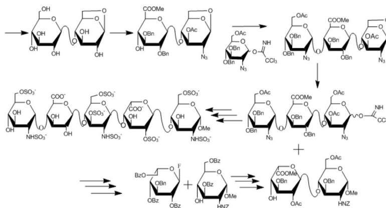
Figure 7. Convergent chemical synthesis of fondaparinux, which resembles the pentasaccharide AT-binding domain of heparin, stabilized as the methyl glycoside.
