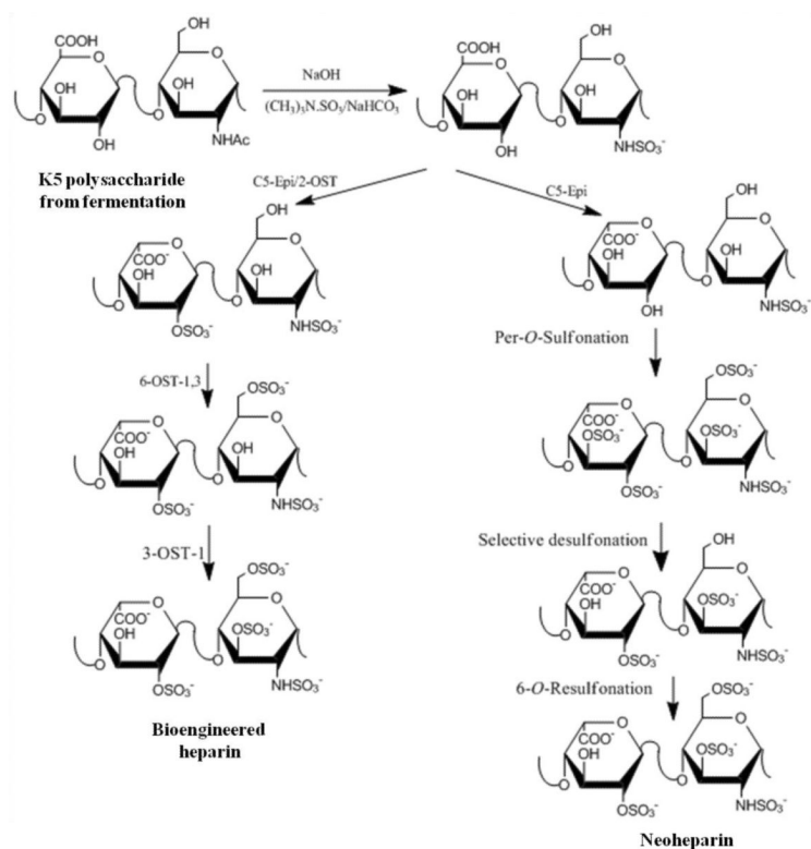
Figure 6. Chemoenzymatic synthesis of heparin and Neoheparin starting from E. coli capsular polysaccharide heparosan. (A) This pathway for the chemoenzymatic synthesis of bioengineered heparin closely resembles the heparin/HS biosynthetic pathway. The chemical de- N -acetylation/ N -sulfonation reaction might be replaced by an enzymatic reaction relying on NDST (B) This pathway for the synthesis of Neoheparin requires selective desulfonation and resulfonation steps and affords some 3- O -sulfo glucuronic acid and iduronic acid residues not found in animal-derived heparin.
