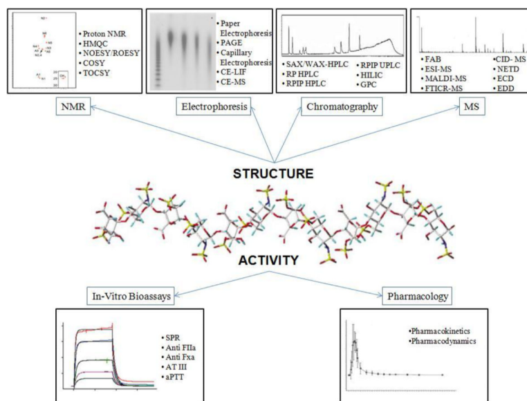
Figure 2. SAR characterization of heparin
