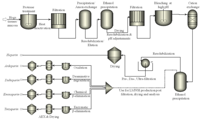
Figure 3. Process flow diagram for production of heparin and LMWHs.
