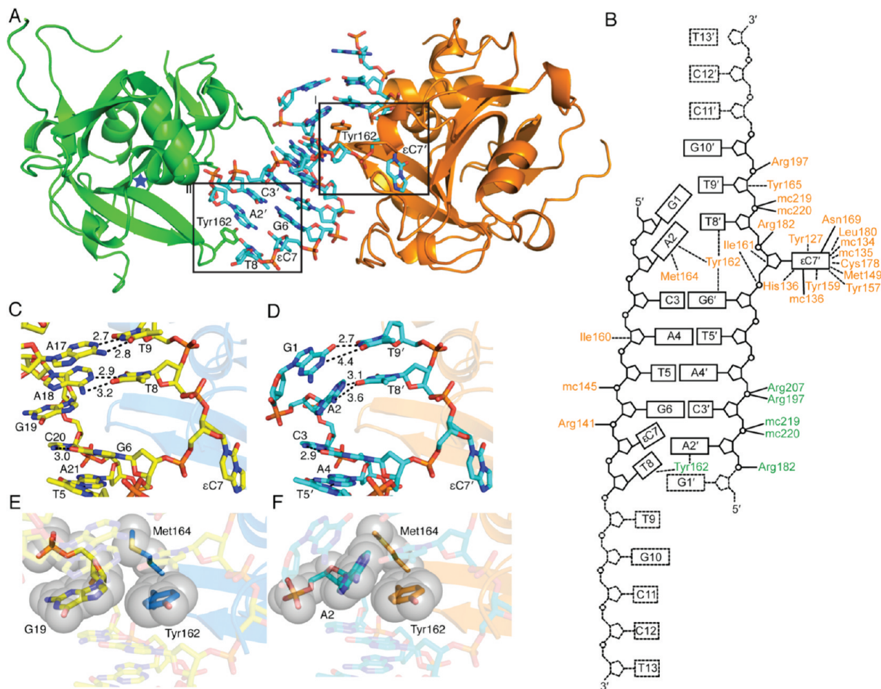
Figure 1. Structures of \Delta 79 AAG bound to \epsilon C DNA. (A) \Delta 79 AAG crystallized in the presence of \text{sseC} DNA has two \Delta 79 AAG molecules in the asymmetric unit: one that makes few contacts with DNA and represents a lower-affinity complex (green) and one that makes multiple contacts with DNA and represents a higher-affinity complex (orange). The two strands of \text{sseC} DNA, which form a pseudoduplex, are shown as sticks with cyan carbons. Panel I displays Tyr162 (orange sticks) intercalating DNA while the \epsilon C lesion is flipped into the active site. Panel II depicts the lower-affinity interaction between \Delta 79 AAG and DNA where Tyr162 (green sticks) stacks with nucleotide A2'. Atoms are colored as follows: red for oxygen, blue for nitrogen, and orange for phosphorus. A blue star denotes the location of the empty active site of lower-affinity AAG. (B) Schematic illustration of the interactions between the two strands of \text{sseC} DNA and amino acid side chains (three-letter code) and main chains (mc) of the \Delta 79 AAG molecules. Amino acid labels from the lower- and higher-affinity (pseudoduplex-bound) \Delta 79 AAG molecules are colored green and orange, respectively. Hydrogen bonds are indicated by solid lines and van der Waals interactions by dashed lines. DNA bases are shown as rectangles containing one-letter codes and numbers that signify their respective positions in the oligonucleotide (5' to 3'). All DNA bases contained in the nucleotide-flipped \epsilon C lesion strand are denoted with a prime. Disordered nucleotides are shown in dashed lines. (C) Nucleotide interactions near the lesion in \Delta 79 AAG- \epsilon C:G dsDNA (PDB entry 3QJ5) (yellow carbons). Relevant distances shown by dashed lines are given in angstroms. (D) Nucleotide interactions near the lesion in the pseudoduplex \Delta 79 AAG structure (cyan carbons). (E) van der Waals interactions with G19 in the \Delta 79 AAG- \epsilon C:G structure. (F) van der Waals interactions with A2 in the pseudoduplex \Delta 79 AAG structure.
