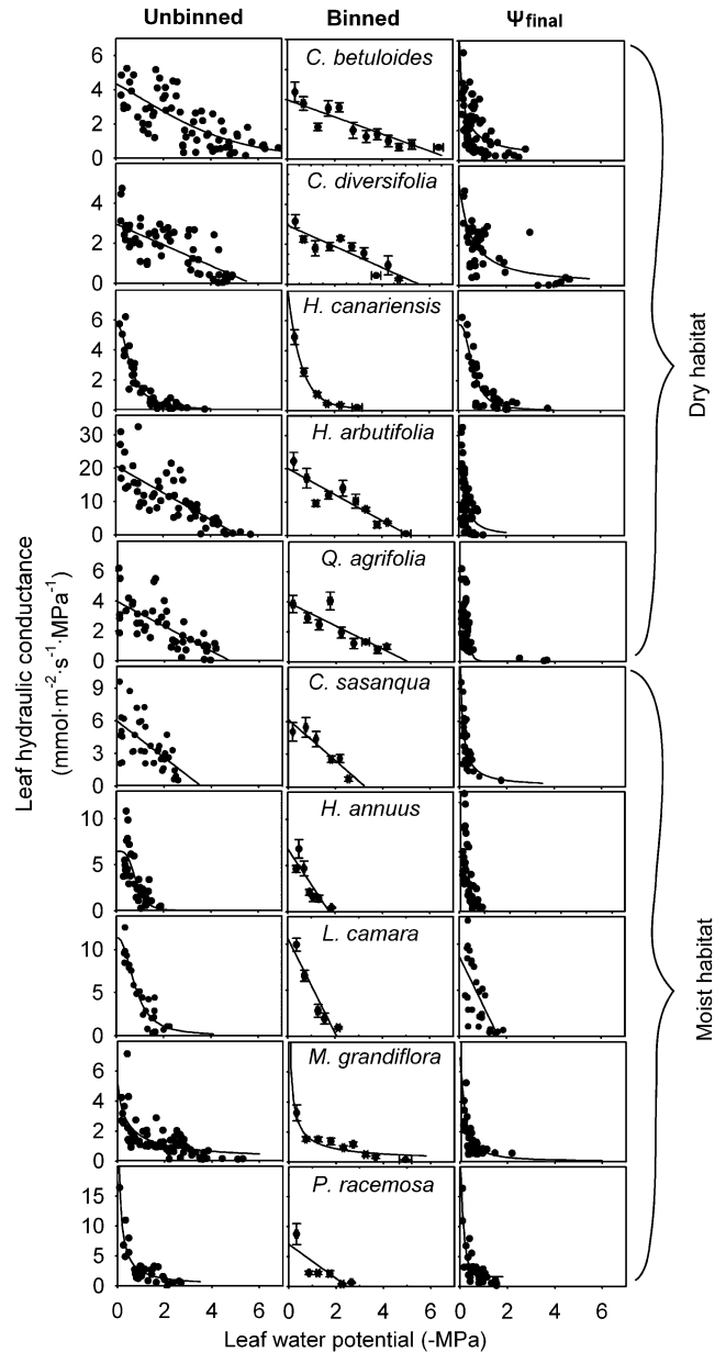
Fig. 2. Vulnerability curves for leaf hydraulic conductance ( K_{\text{leaf}} ) for 10 species varying widely in drought tolerance, determined using the evaporative flux method using three different plots (‘ \Psi_{\text{lowest}} unbinned’, ‘ \Psi_{\text{lowest}} binned’, and ‘ \Psi_{\text{final}} ’). For the ‘ \Psi_{\text{lowest}} unbinned’ and ‘ \Psi_{\text{final}} ’ panels, each point represents a different leaf measured. Standard errors are represented for each bin point in the ‘ \Psi_{\text{lowest}} binned’ plot. The lines plotted are the maximum likelihood functions using each plot for each species (Supplementary Table S3 at JXB online).
