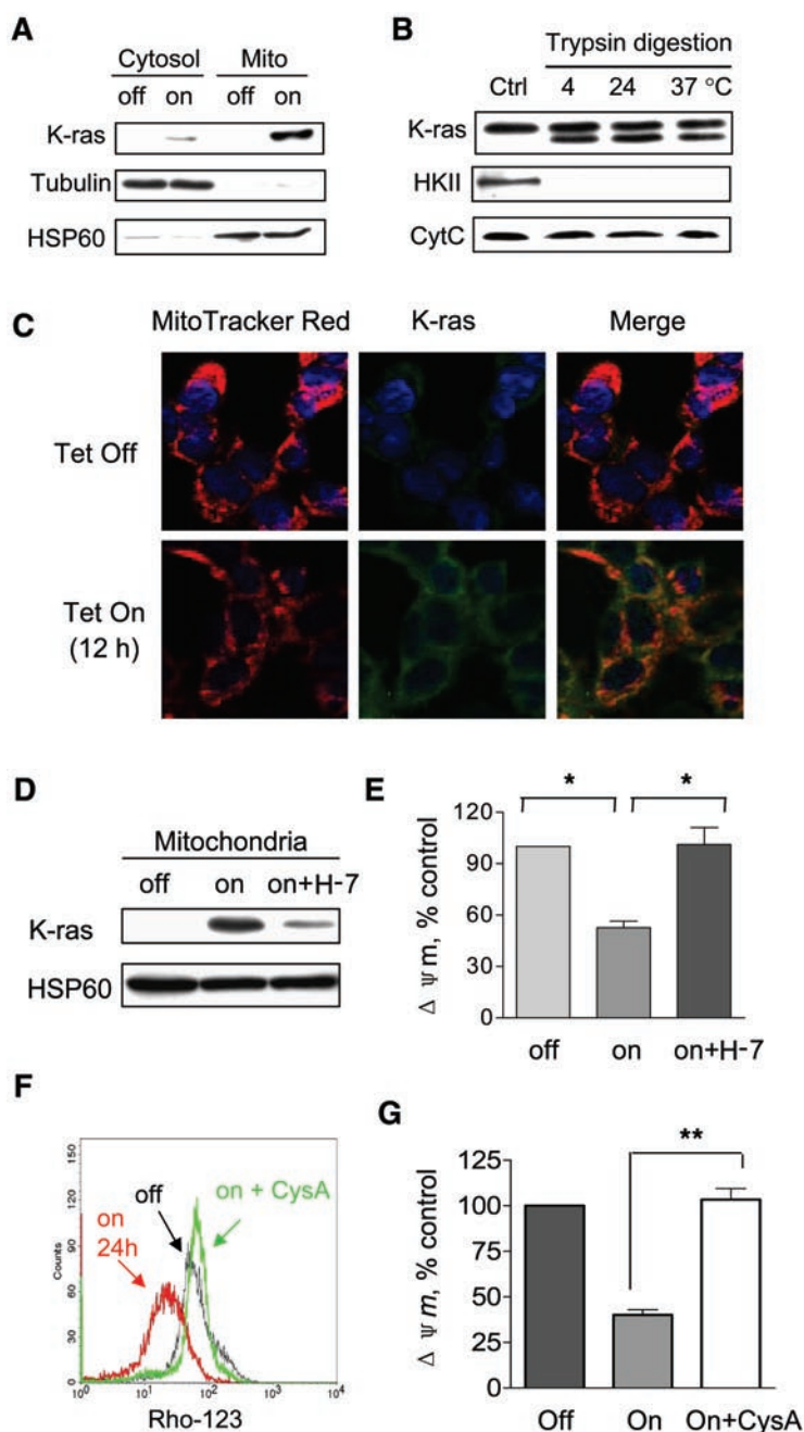
Figure 3 Translocation of K-RAS protein to the mitochondria and its role in causing mitochondrial dysfunction. (A) Mitochondrial fraction was isolated from T-Rex cells before and after doxycycline induction for 12 h. Protein lysates of cytosol and mitochondria (Mito) were analyzed for the presence of K-ras. HSP60 and tubulin were used as mitochondrial and cytosolic markers, respectively. (B) Isolated mitochondria from T-Rex cells with K-ras G12V induction (Control) were treated with 100 \mu g/ml trypsin for 30 min at 4 °C, 24 °C and 37 °C. Western blotting analysis was used to reveal K-ras, hexokinase II (HKII) and cytochrome c. (C) Confocal microscopic analysis of the localization of K-ras. HEK293 cells before and after K-ras induction for 12 h were labeled with MitoTracker Red, K-ras-FITC (green), and DAPI for nuclei (blue) as described in Materials and Methods. (D) Immunoblotting of mitochondrial lysates from T-Rex cells without doxycycline induction (lane 1), with doxycycline induction for 12 h (lane 2), and with doxycycline induction plus 25 \mu M H-7 (lane 3). Translocation of K-ras to the mitochondria was partially prevented by PKC inhibitor H-7. (E) K-ras activation (Tet/on) caused a decrease of mitochondrial transmembrane potential by 50% compared to control (off). Decrease of transmembrane potential was rescued by simultaneous treatment of H-7 (on + H-7). (F) K-ras-induced decrease of transmembrane potential was rescued by treatment with 5 \mu M cyclosporin A (on + CysA). (G) Quantitative analysis of transmembrane potential in K-ras-expressing cells in the presence or absence of cyclosporin A. Data are shown as mean \pm SD. n = 3 , * P < 0.05 , ** P < 0.01 .
