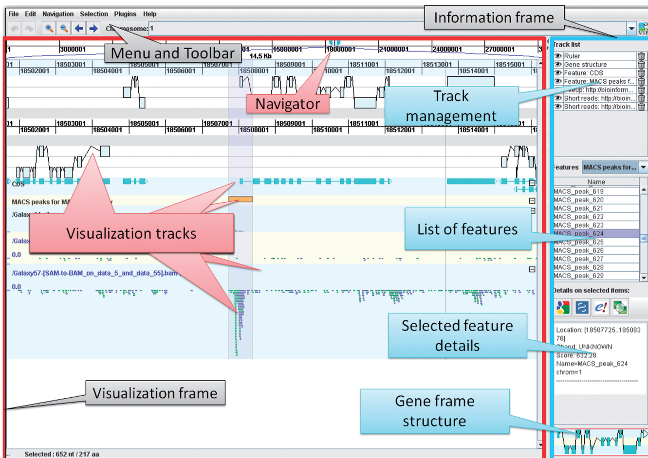
Figure 1. Overview of the GUI layout of GenomeView. The top of the screen displays the menu and toolbar which provide access to all functions of GenomeView. The user interface is divided into two main frames with on the left the visualization frame and on the right the information frame. The visualization frame is further divided into a navigation bar at the top (indicated with 'Navigator'), which allows users to quickly browse through the genome, and a large area that contains the various visualization tracks. The information frame contains four panels that provide management options and information about the data that is currently loaded. Navigation is entirely continuous, in contrast to step-wise navigation found in most other browsers. Furthermore, the zooming is semantic which means that the representation of the data changes according to zoom level and the amount of data on-screen.
