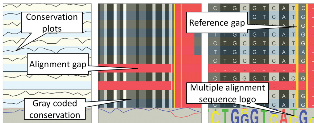
Figure 3. Overview of the basic multiple alignment track. Each line represents another organism. The left panel shows a large area and the multiple alignment tracks show conservation plots between the aligned sequence and the reference. When zooming in (the two rightmost panels), the conservation over the organisms is gray-coded in each track (black=100%, dark gray >75%, light gray >50% and white <50% conservation). Gaps in the aligned sequence are indicated in red, gaps in the reference are indicated with vertical yellow lines. The rightmost zoom is down to the nucleotide level and shows a sequence logo for each position in the alignment.
