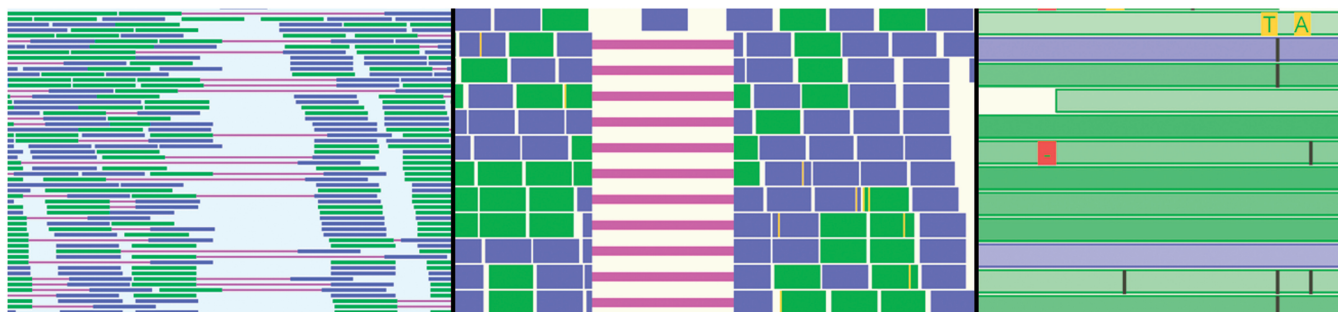
Figure 5. Overview of the short-read visualization track. This track shows the alignment of individual reads. Green and blue indicate reads mapping to the forward and reverse strand respectively. Purple lines are used to connect paired-end reads (left panel), or two parts of a read that has been aligned over a splice-junction (center panel). Yellow indicates mismatches between the read and the reference genome. Black and red are used to indicate indels (right panel). The brightness of the color of a read indicates the mapping quality assigned by the mapping software used in producing this short-read alignment. The lighter a read, the lower the mapping quality. In case of paired-end sequencing there is a second color scheme (not shown) to indicate directionality of the read.
