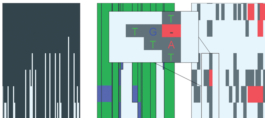
Figure 4. Overview of the advanced multiple alignment track for large genomes. At a high-level perspective (left panel) the histogram-like plot shows the number of segments that align to the corresponding region in the reference genome. Essentially, this is a conservation plot. When zooming in, more details emerge (center panel). The height of the block is still relative to the number of species that contain that particular alignment block. The colors of the lines in each alignment block indicate the strand used in the alignment. Blue segments are aligned to the reverse strand, while green segments are mapped to the forward strand. When hovering over the block, a pop-up will appear that shows the organism name for each line in the alignment block. Zooming in further will provide more detailed information on the multiple alignments (right panel). At this level, mismatches are indicated with gray blocks and gaps with red blocks. When zooming in even further (inset), the gray blocks will contain the letter of the mismatched nucleotide in the aligned organism.
