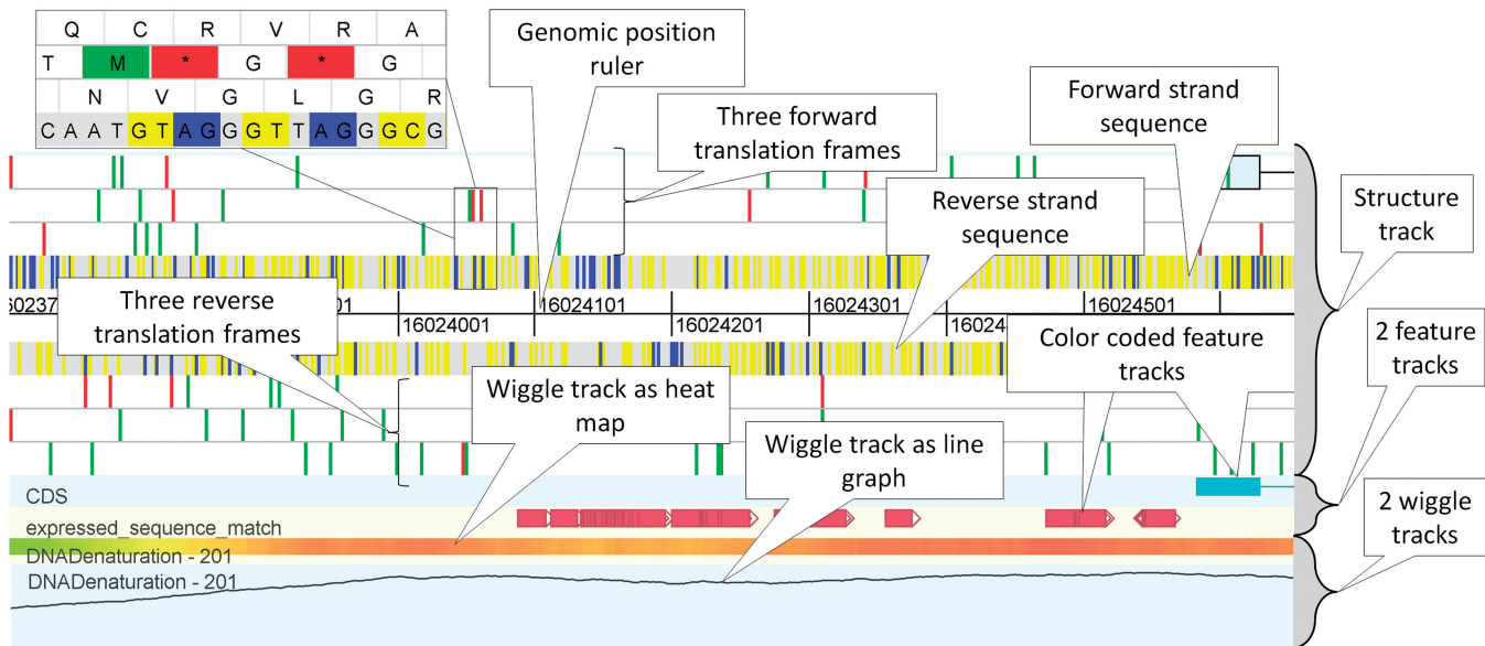
Figure 2. Overview of some standard genome browser tracks. The structure track, which forms the upper part of the figure contains three forward and three reverse translation frames, as well as the forward and reverse strand sequence and the genomic ruler. In the structure track, start and stop codons and splice sites are indicated with a color (see inset for detailed zoom). Beneath the structure track there are two feature tracks that display annotation features using colored blocks. At the bottom of the figure there are two wiggle tracks, one depicted as heat map, the other as a line graph. The data in this figure is part of human chromosome 21, release hg18.
