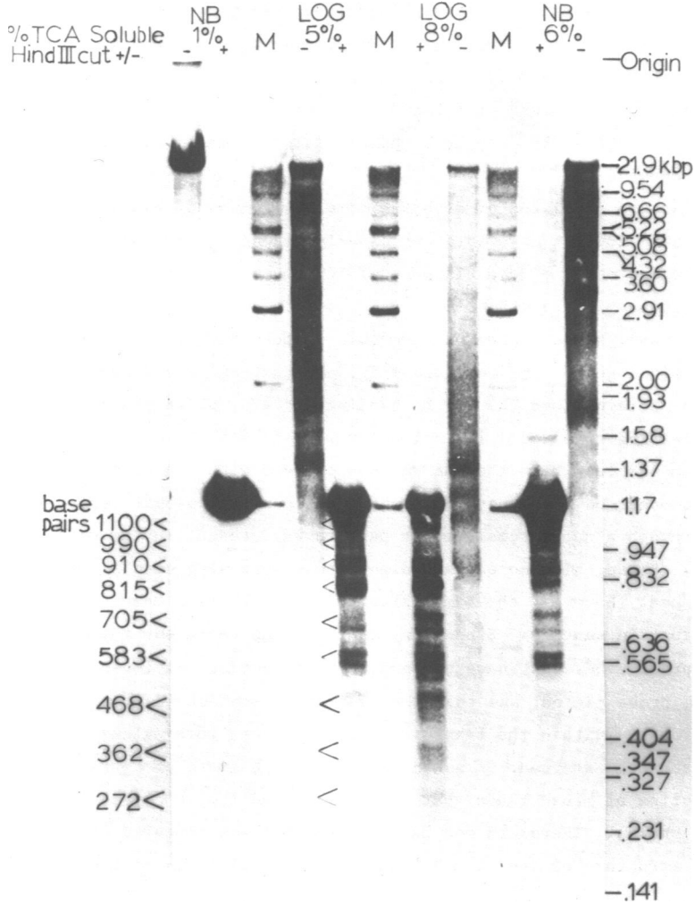
Figure 6. The cleavage pattern of the terminal spacer is dominated by the sequence specificity of the nuclease. DNA derived from micrococcal nuclease digests of log-phase nuclei (log) or of naked bulk DNA (NB) was cut with Hind III (+) or left uncut (-). DNA was then subjected to electrophoresis on a 1.4% agarose gel, transferred to nitrocellulose, and hybridized with the terminal spacer probe. Marker lanes (M) contained an Eco RI-Hind III double digest of \lambda DNA and a Taq I digest of \phi X174 DNA. (<) designates the doublet or triplet bands making up a 100 base pair ladder of nuclease sensitive sites.
