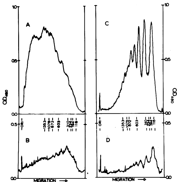
Figure 4. A distinctive nucleosome pattern in the gene region is revealed only after extended nuclease digestion, and more of the DNA is organized in this pattern in starved than in log-phase cells.
