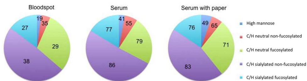
Figure 4. Comparison of N-glycan pattern from serum with and without collection material and dried blood spots
