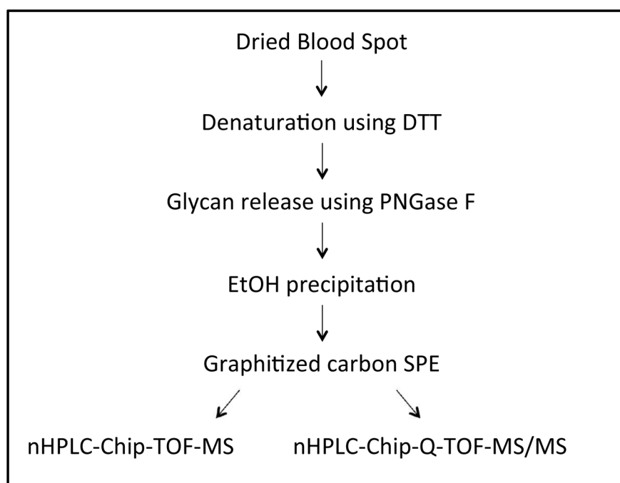
Figure 1. Schematic overview of the procedure for N-glycan analysis of dried blood spots.
