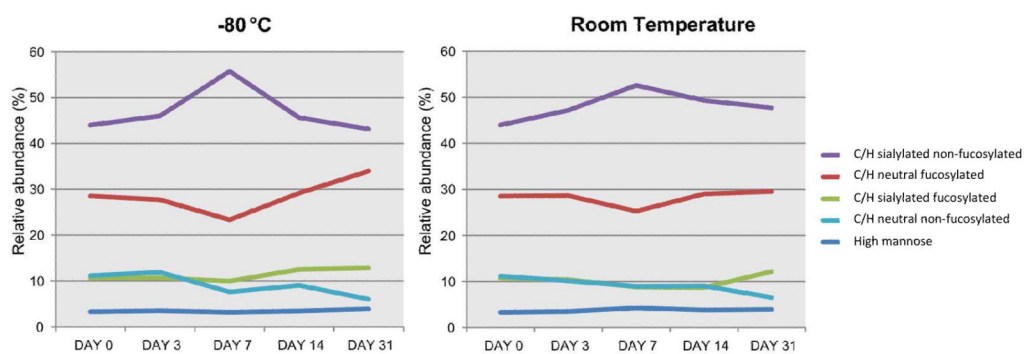
Figure 6. Stability of N-glycans in Dried blood spots during storage
