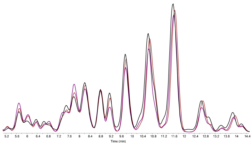
Figure 5. Intra-day variability of the analysis of N-glycans from dried blood spots Three DBS collected from the same individual on the same day were prepared and analyzed on the same day. Extracted N-glycan chromatograms of the three analyses are overlaid to depict the intra-day variability of the analysis
