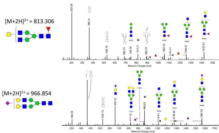
Figure 3. Fragmentation spectra from N-glycans derived from dried blood spots CID fragmentation of N-glycans from DBS obtained from nHPLC-PGC-chip-Q-TOF-MS. * indicates the parent ion. Key: square: N-acetylhexosamine, circle: hexose, red triangle: fucose, blue square: N-acetylglucosamine, green circle: mannose, yellow circle: galactose, purple diamond: sialic acid, Red: reducing end. The structures represented in color have the reducing end present, facilitating their annotation. When the reducing end is not present, it is not possible to distinguish between galactose and mannose residues, therefore, these structures are represented with symbols only.
