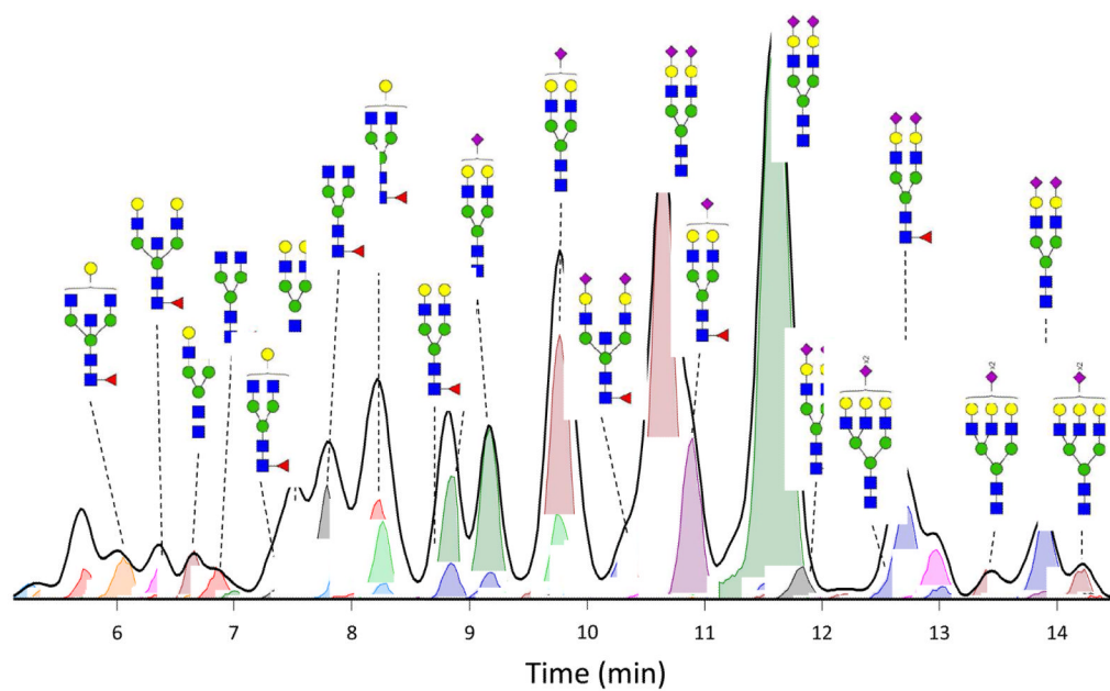
Figure 2. Extracted N-glycan chromatogram and extracted Compound Chromatograms of N-glycans derived from dried blood spots
