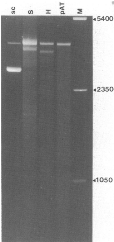
Figure 5: Bromoacetaldehyde modification of pIRbke8 and its parent plasmid pAT153. pIRbke8 was reacted with bromoacetaldehyde followed by restriction cleavage with S alI (S) or H indIII (H). pAT153 (pAT) was analogously treated as in (H). sc, supercoiled pIRbke8; M, phage PM2 digested by H indIII.
