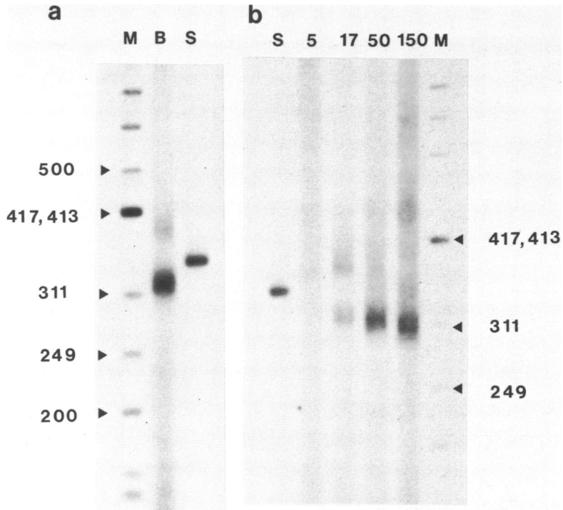
Figure 6: Finer mapping of modification - cleavage pattern in pColIR215. (a) Comparison of S1 and bromoacetaldehyde targets. Autoradiograph of 5% polyacrylamide gel electrophoresis of [5',-^{32}P] labelled -340bp fragments arising from S1, Bam HI cleavage (S) or bromoacetaldehyde (25mM), Bam HI, S1 cleavage (B). M, phage \phi X174RF DNA digested by Hinf I and exchange labelled with [^{32}P] as marker fragments. (b) Modification pattern as a function of bromoacetaldehyde concentration, M and S as in (a); other tracks, modification by indicated millimolarity of bromoacetaldehyde.
