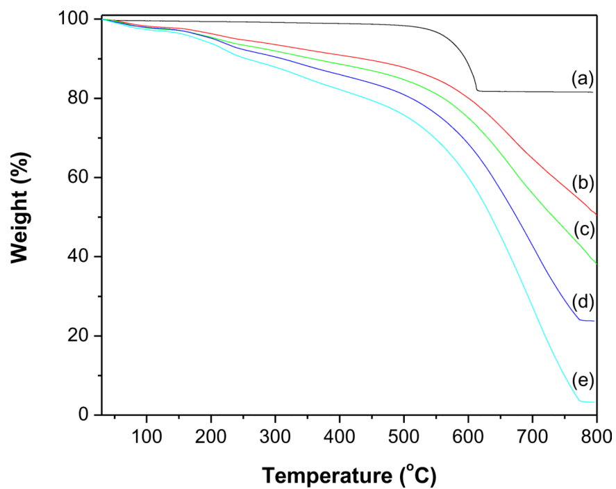
Fig. 5. TGA profiles of (a) MWCNTs-COOH (b) f -MWCNTs/G1 (c) f -MWCNTs/G2 (d) f -MWCNTs/G3 and (e) f -MWCNTs/G4 or f -MWCNTs.
