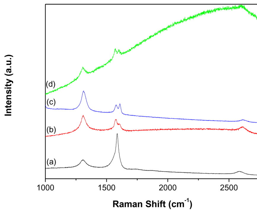
Fig. 4. Raman spectra of (a) p -MWCNTs (b) f -MWCNTs (c) f -MWCNTs-CdS nanocatalyst and (d) f -MWCNTs-Ag 2 S nanocatalyst.
