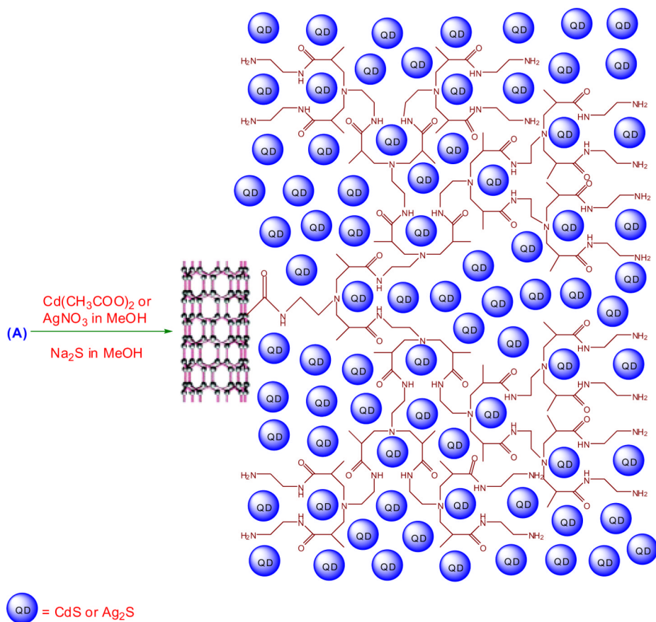
Scheme 2. Deposition of CdS and \text{Ag}_2\text{S} QDs on f -MWCNTs.
