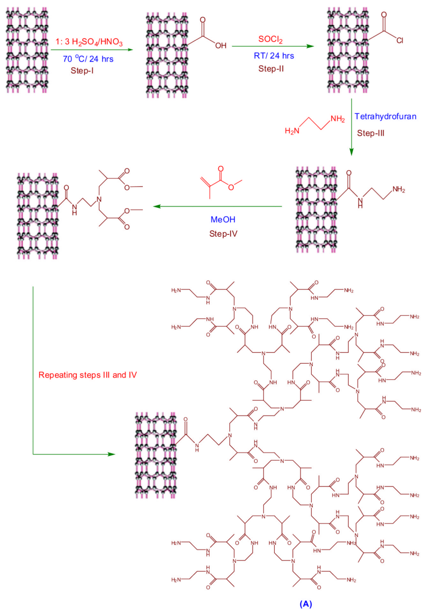
Scheme 1. Covalent grafting of PAMAM dendrimers onto MWCNTs.
