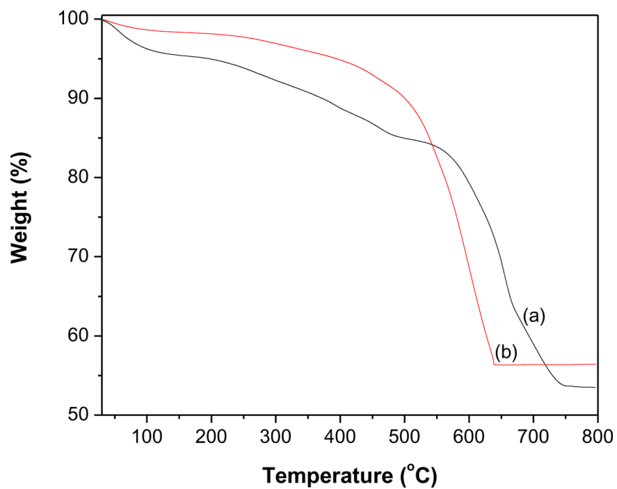
Fig. 6. TGA profiles of (a) f -MWCNTs-CdS nanocatalyst and (b) f -MWCNTs-Ag 2 S nanocatalyst.
