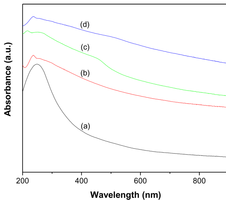
Fig. 1. UV-vis absorption spectra of (a) MWCNTs-COOH (b) f -MWCNTs (c) f -MWCNTs-CdS nanocatalyst and (d) f -MWCNTs-Ag 2 S nanocatalyst.
