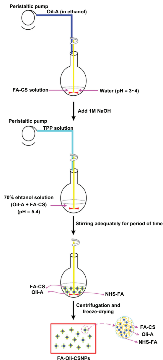
Figure 1 Schematic description of the preparation procedure of FA-Oli-CSNPs. Abbreviations: Oli-A, oligomycin-A; FA-CS, the folate-conjugated chitosan; TPP, sodium tripolyphosphate; FA-Oli-CSNPs, folate-conjugated chitosan nanoparticles loading oligomycin-A; NHS-folate, N-Hydroxysuccinimide ester of folate.
