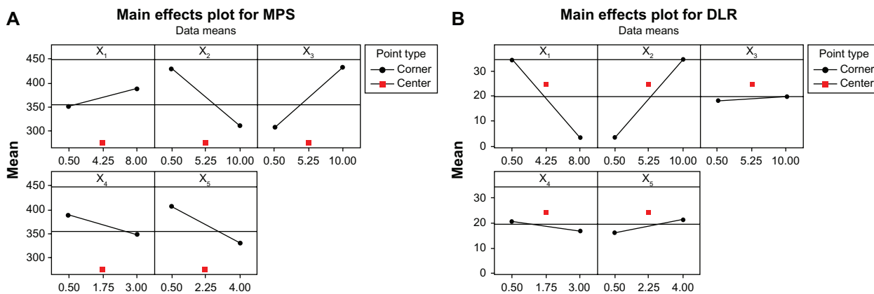
Figure 6 Main effects plot for (A) MPS and (B) DLR. Abbreviations: MPS, mean particle size; DLR, drug loading rate.
