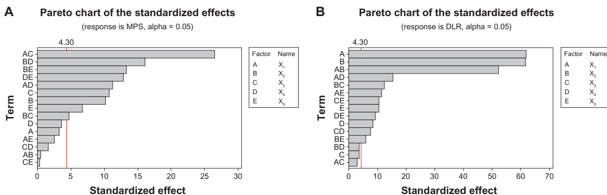
Figure 4 Pareto chart of the standardized effects for (A) MPS and (B) DLR – full model. Abbreviations: MPS, mean particle size; DLR, drug loading rate.
