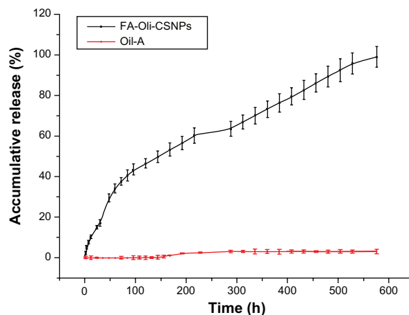
Figure 11 FA-Oli-CSNPs accumulative drug release profile. Abbreviation: FA-Oli-CSNPs, folate-conjugated chitosan nanoparticles which encapsulate oligomycin-A.
