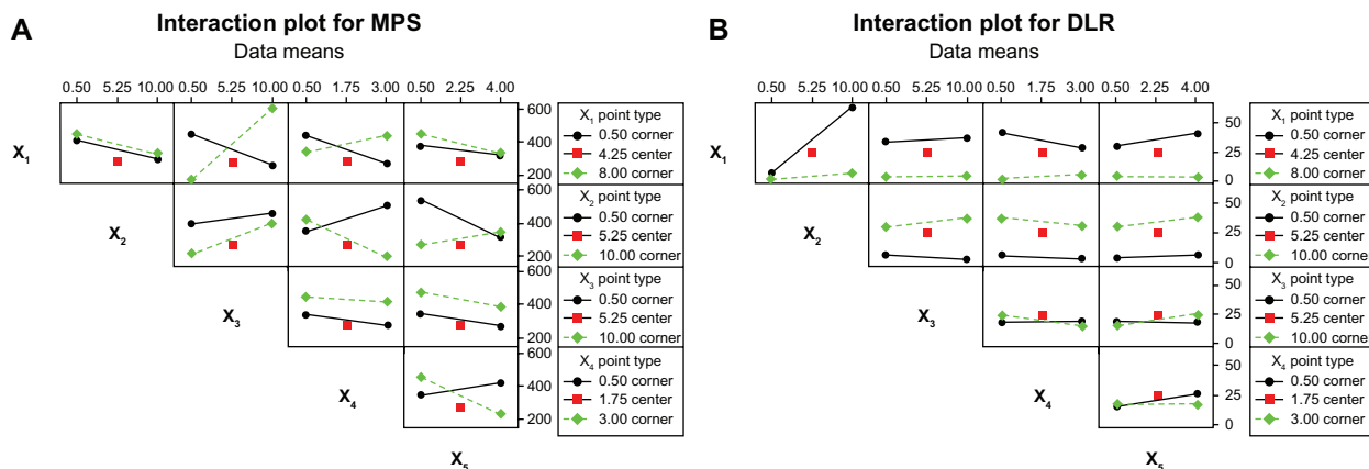
Figure 7 Interaction plot for (A) MPS and (B) DLR. Abbreviations: MPS, mean particle size; DLR, drug loading rate.
