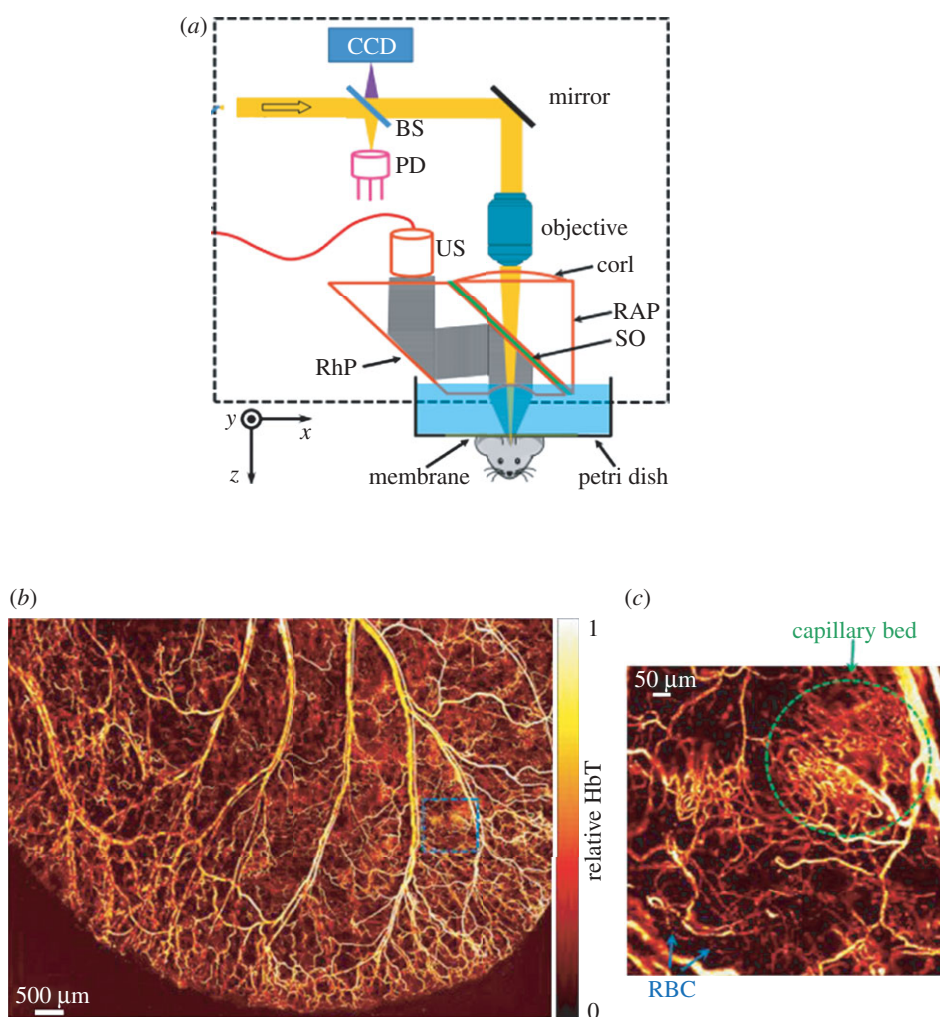
Figure 11. Optical-resolution photoacoustic microscopy (OR-PAM) scanner used for in vivo imaging of the mouse ear [118]. (a) Schematic of system BS, beam splitter; PD, photodiode; CorL, correction lens; RAP, right-angle prism; SO, silicone oil; RhP, rhomboid prism; US, ultrasonic transducer (50 MHz). The CCD is used to view the imaging region. The components that lie within the dotted rectangle form the scan head, which is mechanically translated in order to acquire an image. (b) In vivo image of the microvasculature in the mouse ear. (c) Expanded region shows capillary network and red blood cells (RBC) within a capillary. Excitation wavelength: 570 nm.
