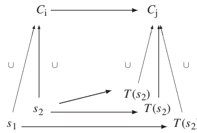
Figure 3. Micro-indeterminism induces deterministic macro-dynamics.
