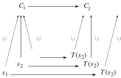
Figure 1. Micro-determinism induces indeterministic macro-dynamics.
