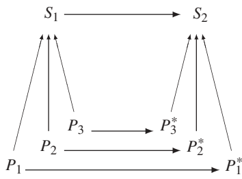
Figure 2. Fodor's hope: meshing dynamics.
