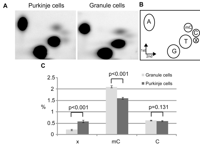
Fig. 1. Quantification of mC and “x” abundance in Purkinje and granule neurons. A , 2D TLC separation of nucleoside monophosphates from genomic DNA in Purkinje and granule cells. B , reference map to the TLC spots (A is dAMP, etc.) (14), with added “x” position. C , percentage shows the abundance of a nucleotide neighboring G. Error bars show SEM (n=11), p values were derived from Matt-Whitney statistics. Neither abundance of dTMP or dAMP were different between the samples (p=0.743 and p=0.793 respectively).
