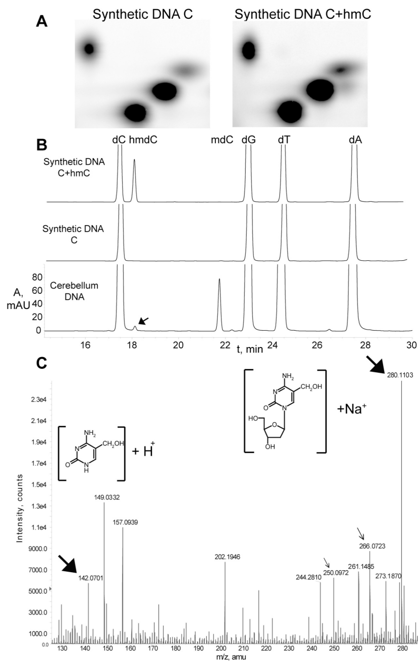
Fig. 2. 2D TLC, HPLC and MS identification of hmC. A , 2D TLC analysis of synthetic DNA templates indicates that hmC comigrates with the “x” spot (Fig 1). B , HPLC chromatograms (A, 254 nm) of the nucleosides derived from synthetic and cerebellum DNA. The peaks were identified using MS. The black arrow points to the peak, which elutes at the same time as hmdC. C , MS of the fraction corresponding to the HPLC peak indicated above. Closed black arrows indicate the masses of 5-hydroxymethylcytosine and 5-hydroxymethyl-2'-deoxycytidine sodium ions (structures are shown on the insets). Open arrows indicate the ions generated by 2'-deoxycytidine, which elutes in a large nearby peak and spills over into the analyzed fraction.
