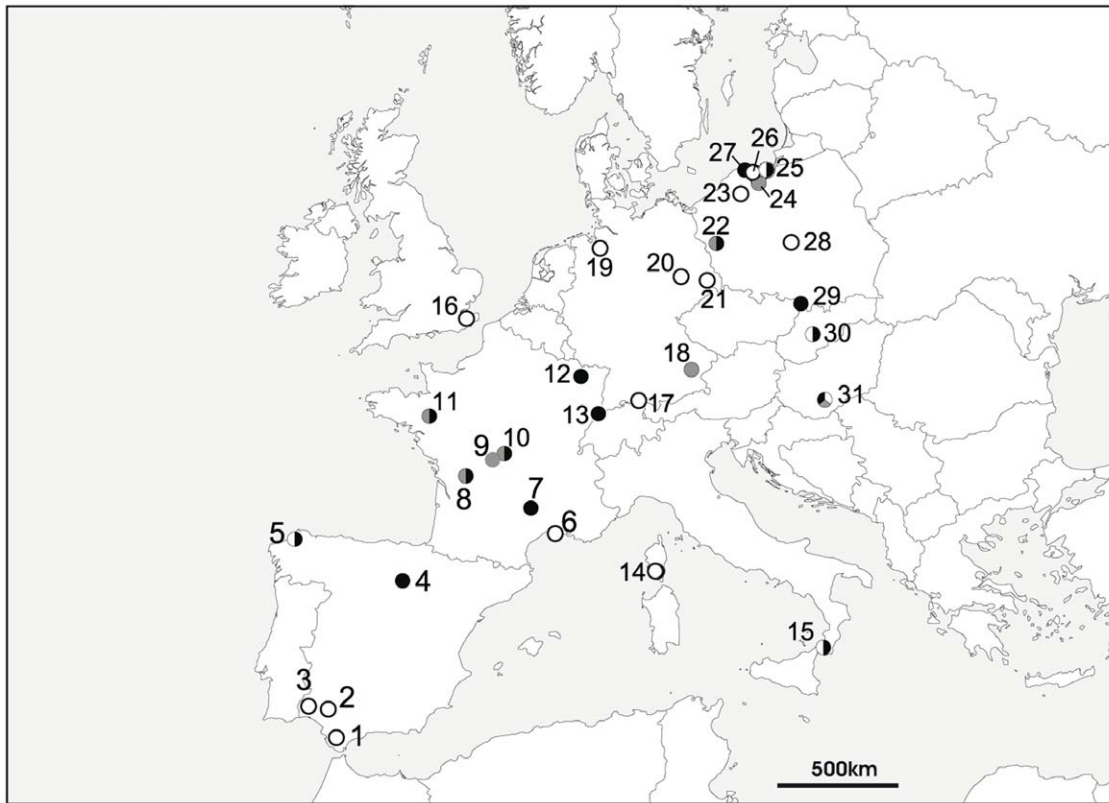
Figure 1. Site locations of bat hair samples. Circles are filled in according to the species or genus at that site: Eptesicus serotinus / E. isabellinus , open circles; Barbastella barbastellus , grey circles; Plecotus auritus / P. austriacus , black circles. Proximate sampling sites were grouped as one circle for clarity. Numbers refer to sites in Table S1. doi:10.1371/journal.pone.0030388.g001
