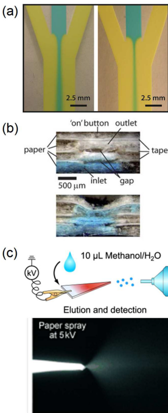
Figure 5. Paper microfluidics. Recent advances in this area include (a) recapitulation of fluid handling functionalities from traditional microfluidics, including laminar focusing, (b) integration of programmable switches, and (c) coupling to mass spectrometry using paper spray. (a) Laminar focusing was demonstrated in a paper device. (b) Tape and paper were used to fabricate a programmable 3D paper device. When the “on” button was depressed, a new flow path formed. (c) Analytes from whole blood were electrospayed directly from paper. Figures reproduced with permission from references 81, 85 and 38.
