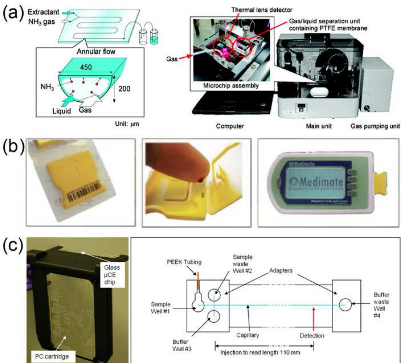
Figure 7. MicroTAS. True \mu\text{TAS} systems have been developed for (a) ammonia gas monitoring in clean rooms, (b) point-of-care determination of lithium in blood, and (c) forensic DNA analysis. (a) Annular flow extracted \text{NH}_3 gas for colorimetric determination in the control and detection system shown to the right. (b) A sealed cartridge accepted whole blood for electrophoretic separation and electrochemical detection of lithium levels. (c) DNA was extracted from buccal swabs and amplified by PCR in the polycarbonate (PC) cartridge, then transferred to the glass chip for separation and detection. Figures reproduced with permission from references 125, 129 and 143.
