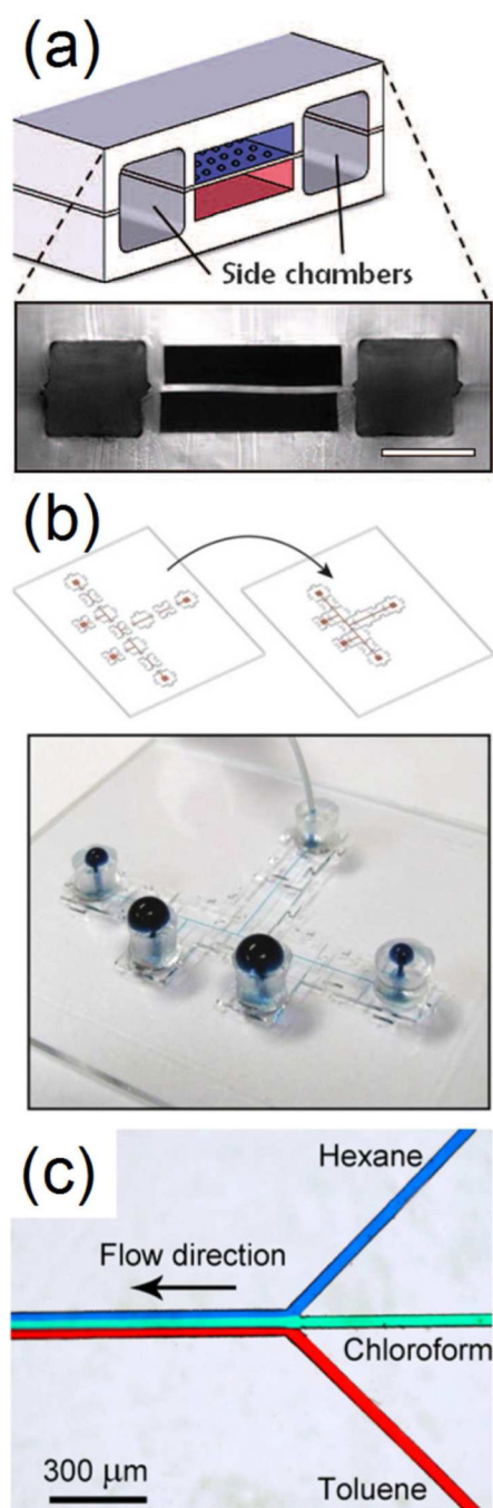
Figure 2. Microfabricated devices. Recent advances in microfabrication include (a) improved replication of in vivo conditions, (b) development of modular units, and (c) the use of solvent-resistant materials. (a) A lung-on-a-chip microfluidic device was composed of two large side chambers and a central microchannel separated by a 10- \mu\text{m} thick porous PDMS membrane. Scale bar, 200 \mu\text{m} . (b) A selection of pre-fabricated microfluidic assembly blocks were produced (top left), followed by assembly and bonding (top right) into a complete device (bottom). (c) A whole-Teflon microfluidic chip showed robust solvent compatibility using laminar flow of dyed organic solvents. Figures reproduced with permission from references 4, 9 and 10.
