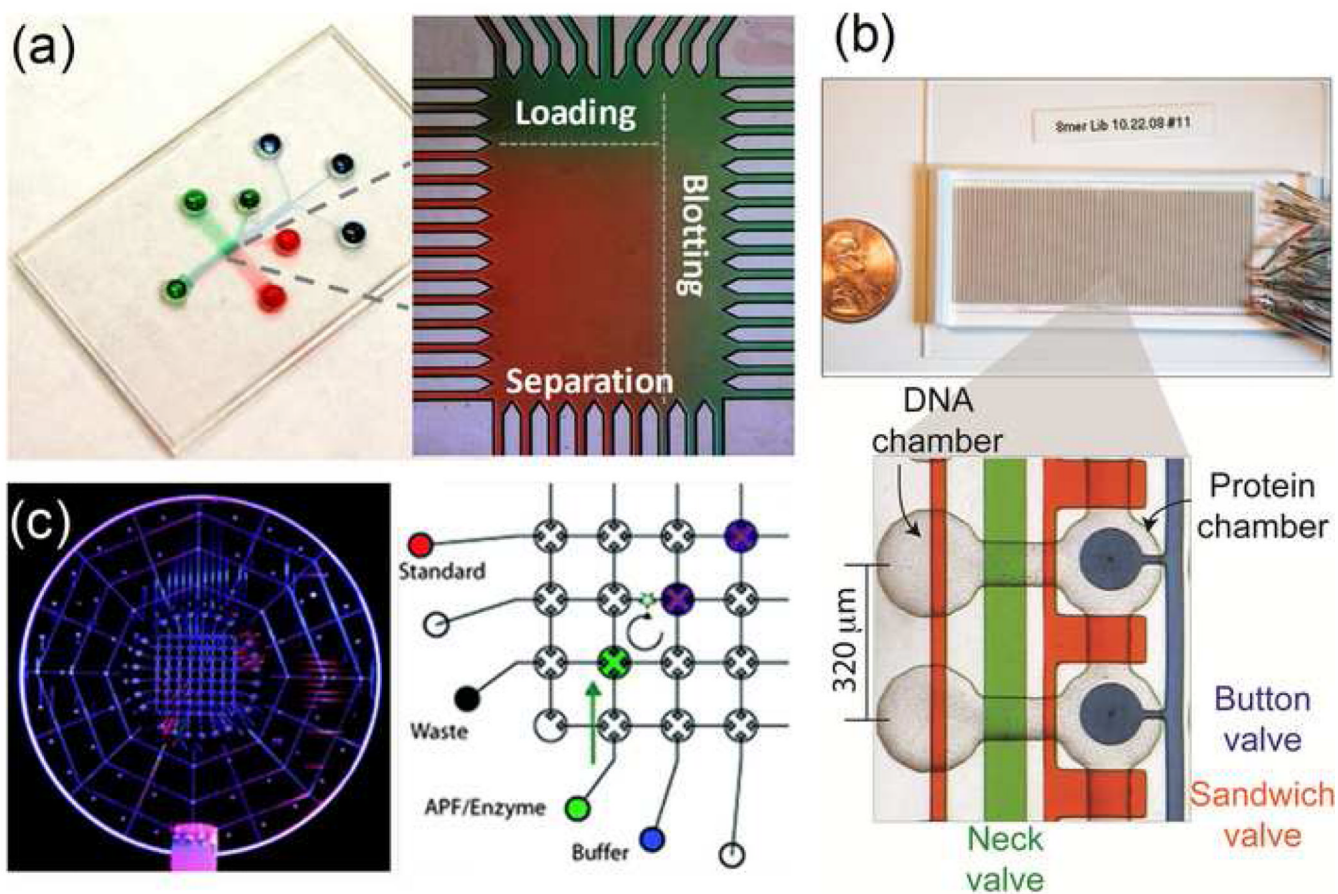
Figure 6. Rapid analyses. Microfluidic devices dramatically increase the speed at which biochemical information can be obtained by (a) decreasing analysis time, (b) multiplexing, and (c) automation. (a) A microfluidic device for western blotting cut analysis time to just 5 min using a discontinuous gel. (b) A massively parallel device screened transcription factor binding using arrays of valves. (c) A third device automated biochemical assays, including generation of a standard curve and sample analysis. Figures reproduced with permission from references 92, 102 and 63.
