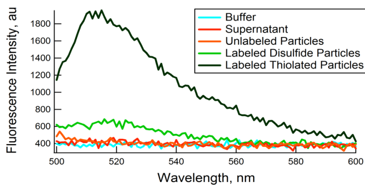
Figure 3. Fluorescence spectra ( \lambda_{ex} = 494 nm) of (dark green) fluorescein-labeled pNIPMAM-BAC-Bis particles, (orange) unlabeled particles, (blue) pH 7.4 HEPES buffer, and (red) the supernatant following purification by centrifugation. Particles that were not reduced and therefore retained their disulfide linkages (light green) had much lower coupling efficiency than that of the reduced particles.
