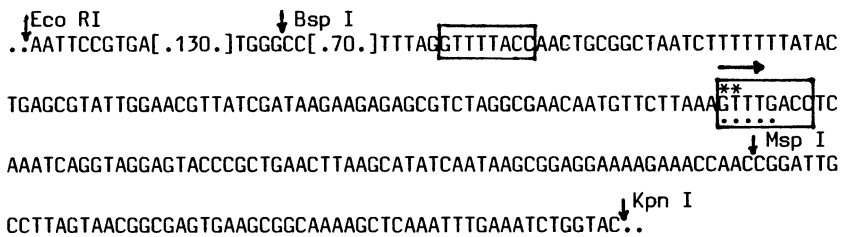
Figure 4. Primary structure ( non-coding strand ) of part of the Eco RI-Kpn I subfragment of the Eco RI-A fragment showing the location of the 5'-end of 25 S rRNA ( horizontal arrow ). The nucleotides marked by . and * are identified as corresponding to the 5'-terminus of 25 S rRNA by nuclease S 1 mapping ( . ) or by reverse transcriptase extension ( * ), respectively. The octanucleotide repeat located at the 5'-end of 25 S rRNA and 92 nucleotides upstream is boxed.
