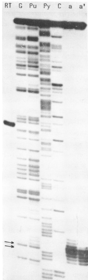
Figure 5. Identification of the 5'-terminus of the 25 S rRNA gene. Right - Mapping of nuclease S_1 protection products of the hybrids between 25 S rRNA and the Bsp I-Msp I subfragment of fragment Eco RI-Kpn I (see Figs 1 & 4). The hybrids are digested with 5 [a] and 25 [a'] units of nuclease S_1 and run in parallel with a Maxam and Gilbert ( 13 ) sequence ladder of the same rDNA subfragment. Left - Reverse transcriptase extension product of the Msp I-Kpn I subfragment of fragment Eco RI-Kpn I hybridized with 25 S rRNA. The horizontal arrows indicate the position of the 5'-terminus nucleotides of 25 S rRNA on the ladder of the Bsp I-Msp I subfragment after correction for the size of the Msp I-Kpn I subfragment (52 nucleotides in the coding strand) used as primer.
