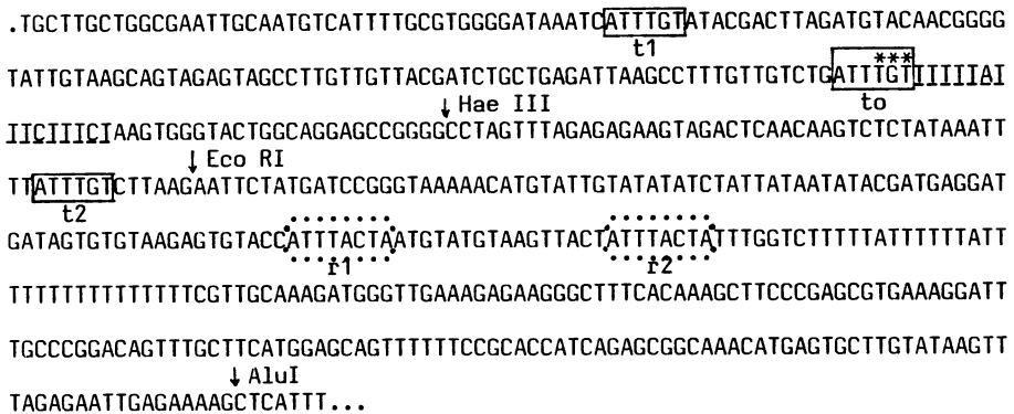
Figure 6. Primary structure ( non-coding strand ) of the parts of Eco RI-E and Eco RI-B fragments encompassing the 3'-terminus of the 25 S rRNA gene. The nucleotides marked by * are identified as corresponding to the 3'-terminus of 25 S rRNA ( see text and Fig.7 ). The boxes to, t1 and t2 designate a hexanucleotide repeat found at the distal end of fragment Eco RI-E. The octanucleotide repeat r1 and r2 marks the position of a 24 nucleotide insertion not encountered in previous structural studies on a different yeast rDNA clone. Terminal nucleotides found in 37 S pre-rRNA are underlined.
