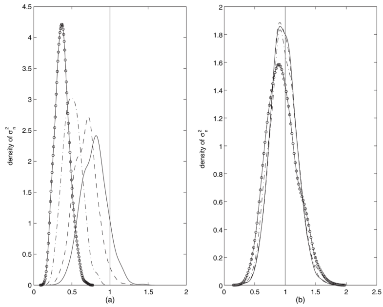
Fig. 3. (a) Densities of the variance estimators based on the naive two-stage approach for various numbers of spurious variables and (b) densities of RCV estimators of variance (all calculations are based on 500 simulations using SIS as a model selector and the sample size n is 50; they show that the biases of the naive two-stage estimator are correctable): |, true variance 1; —, s = 1 ; ---, s = 2 ; · · · · ·, s = 5 ; —○—, s = 10
