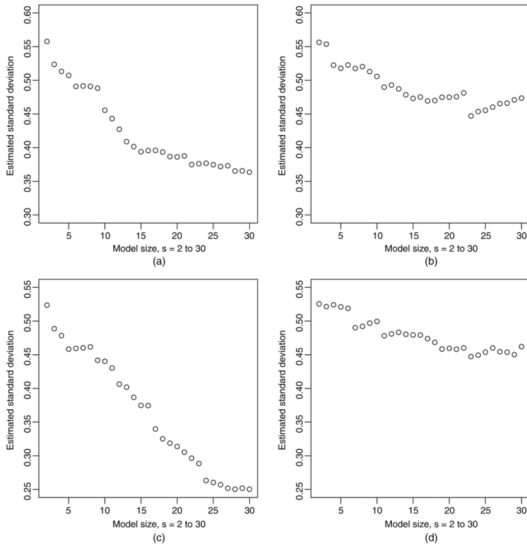
Fig. 10. Estimated standard deviation of benchmark one-step forecast of HPA in San Francisco and Los Angeles for various model sizes: (a) San Francisco, naive method; (b) San Francisco, RCV method; (c) Los Angeles, naive method; (d) Los Angeles, RCV method
