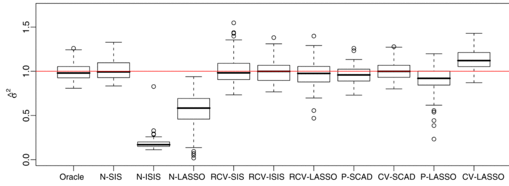
Fig. 5. Comparison of various methods for variance estimation in model (18) with n = 200 and p = 2000 ( \rho = 0.5 and b = 1 ): presented are boxplots of \hat{\sigma}_n^2 based on 100 replications
