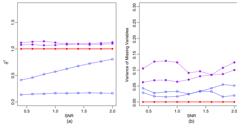
Fig. 9. (a) Medians of various variance estimators when n = 400 and p = 10000 among 100 replications (●, oracle; ○, N-SIS; □, N-ISIS; ●, RCV-SIS; ■, RCV-ISIS) and (b) medians of variance of missing variables of various model selection tools (●, oracle; ○, SIS; □, ISIS; ●, RCV-SIS; ■, RCV-ISIS)
