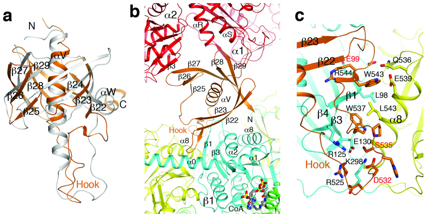
Figure 3. The BT domain mediates interactions in the MCC holoenzyme (a). Overlay of the structure of PaMCC BT domain (in orange) with that of PCC (gray). A large conformational difference for the hook is visible. The exact positions of many of the \beta -strands are different as well. (b). The BT domain (orange) contacts a \beta subunit ( \beta 1 , N domain in cyan, C domain yellow) as well as a neighboring \alpha subunit ( \alpha 2 , red) in the PaMCC holoenzyme. (c). Detailed interactions between the hook of the BT domain and the \beta subunit in PaMCC. Three disease-causing mutation sites near this interface are labeled in red. For stereo version of the panels, please see Supplementary Figs. 9, 10.
