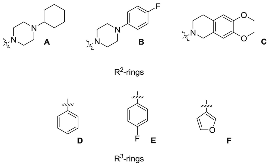
Figure 2. R 2 - and R 3 -rings
