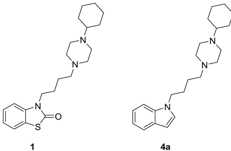
Figure 1. Structures of 1 and its indole analogue 4a
