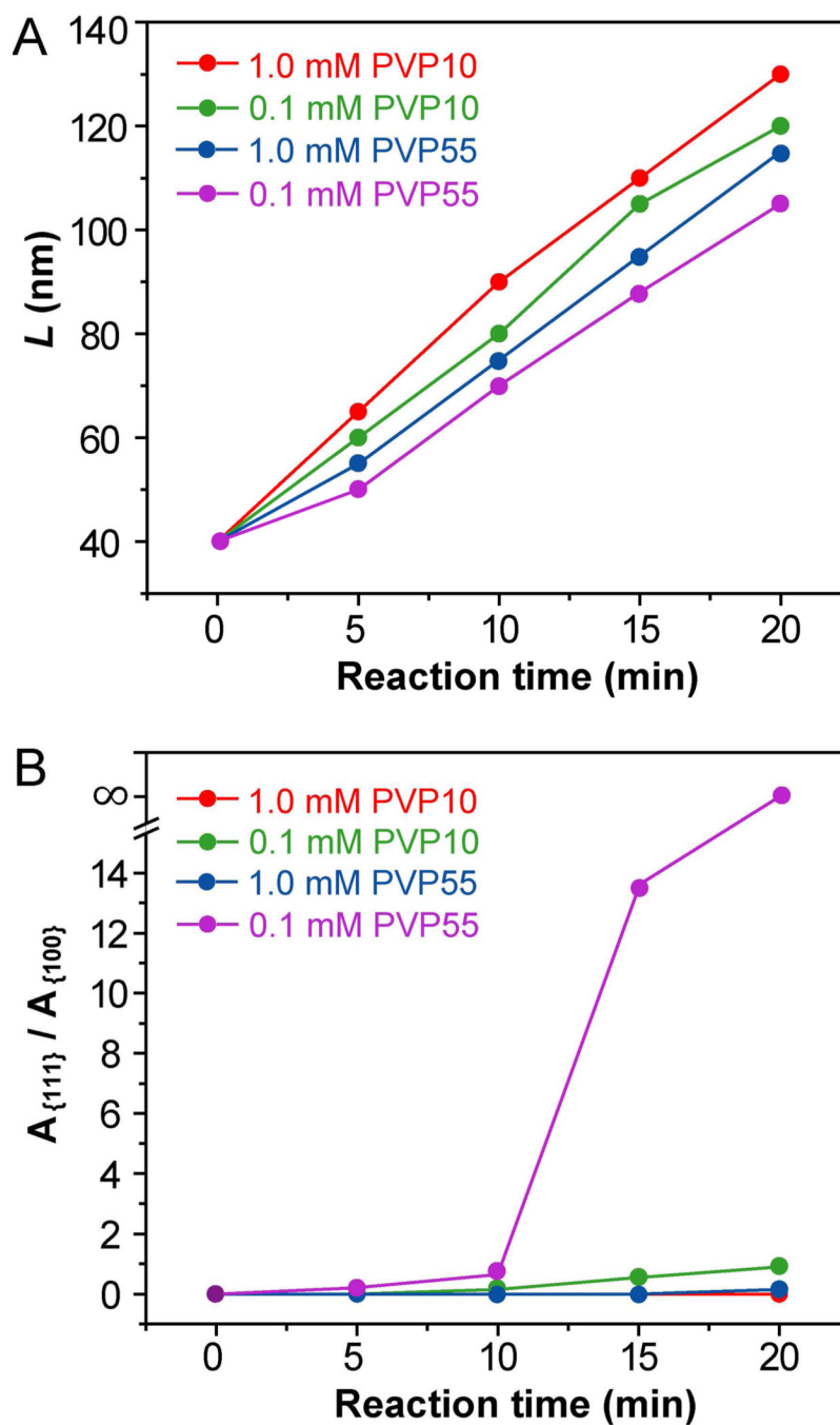
Figure 7. Plots of (A) the size ( L ) and (B) the ratio between areas of {111} and {100} facets (denoted as A_{\{111\}} and A_{\{100\}} , respectively) for the Ag nanocrystals shown in Figures 2 and 4 as a function of reaction time.
