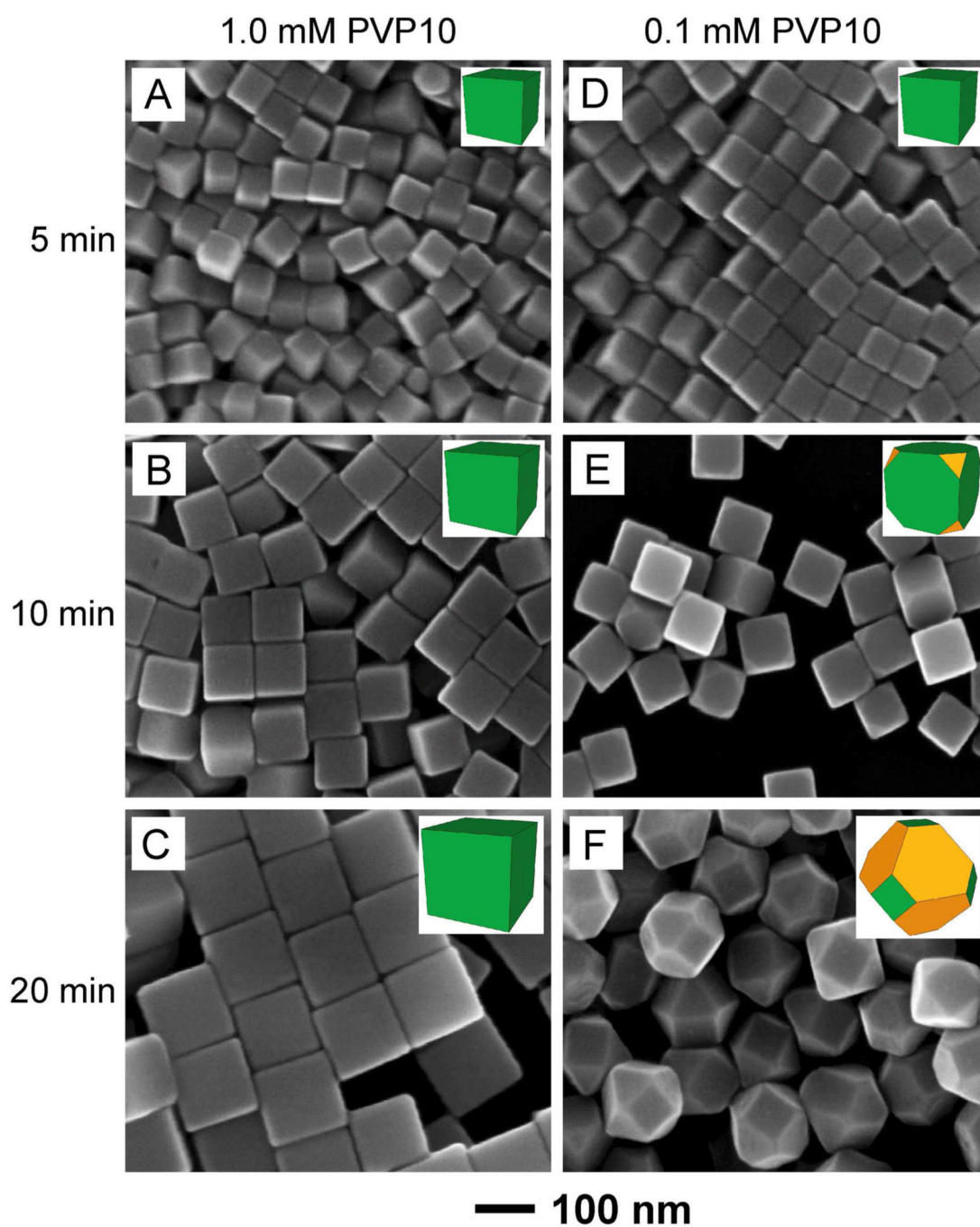
Figure 4. SEM images of Ag polyhedrons grown from 40-nm cubic seeds in the presence of (A–C) 1.0 mM and (D–F) 0.1 mM PVP10 as the capping agent. The samples were collected from the reaction solutions at different reaction times: (A, D) 5 min, (B, E) 10 min, and (C, F) 20 min. The inset shows the corresponding 3D model for each type of polyhedron.
