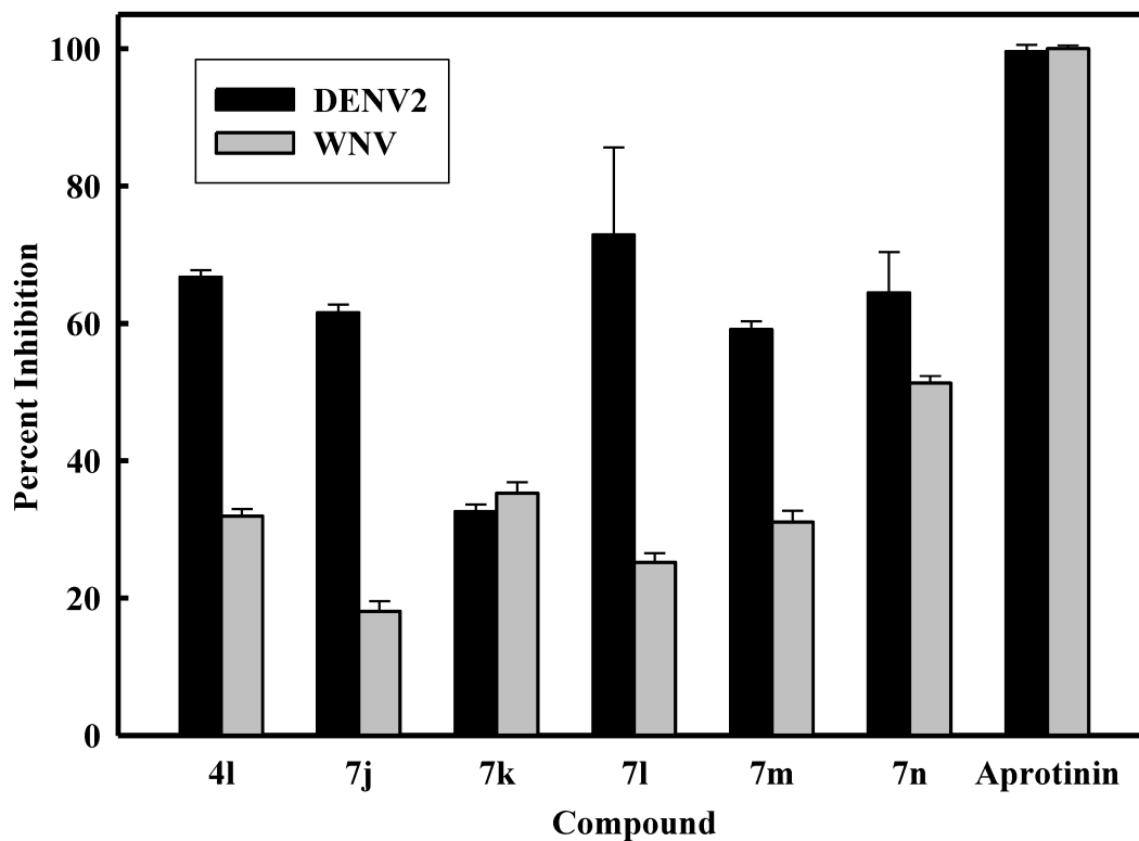
Figure 3. Inhibition of DENV2 and WNV NS2B-NS3pro by selected derivatives of (I-II) at 25 \mu M. The concentrations of DENV2 and WNV NS2B-NS3 proteases were 25 nM and 28 nM, respectively. The buffer used contained 200 mM Tris hydrochloride, 6 mM NaCl, and 30% glycerol and 0.1% CHAPS, pH 9.5. The percent values were calculated from the relative fluorescence units obtained in the presence and absence of tested compound. All assays were performed in triplicate and the average values are shown. The assays were performed as described in the Biochemistry methods section.
