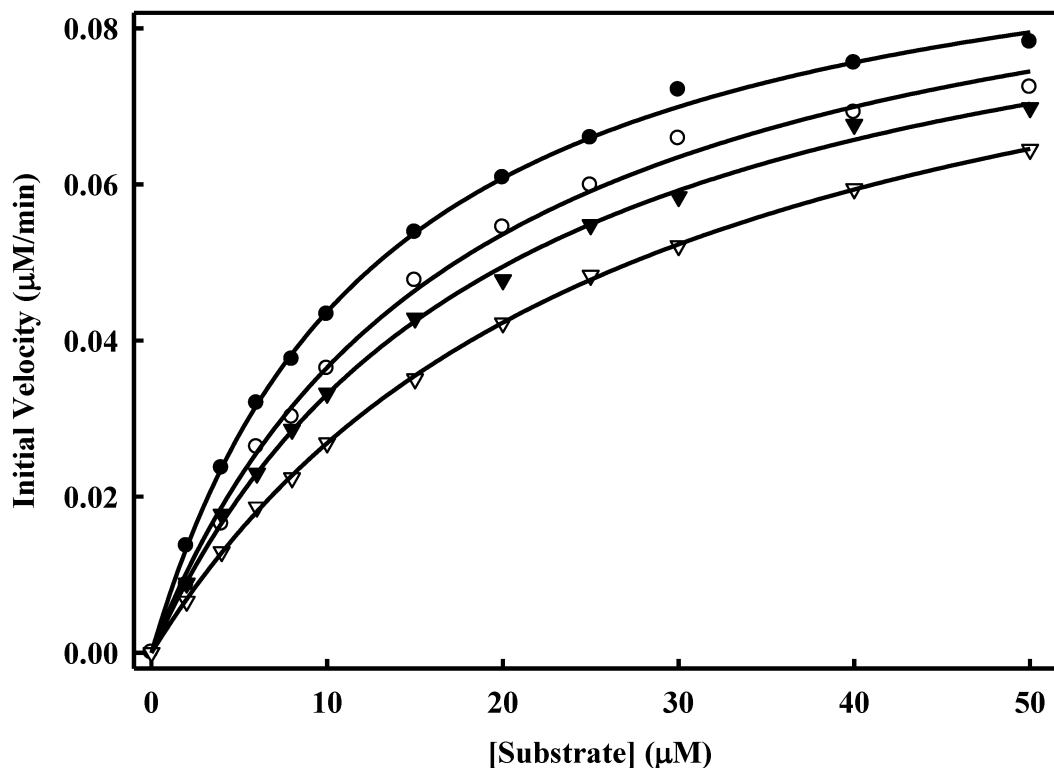
Figure 5. DENV2 NS2B-NS3pro activity in the absence and presence of inhibitor 7n . The in vitro protease assays were performed as described in the Experimental Section. The initial reaction rates of the tetra -peptide substrate cleavage catalyzed by 0.025 μM DENV2 NS2B-NS3 protease in the absence (●)-(●) and the presence of 1.0 μM (○)-(○), 2.0 μM (▼-▼) and 5.0 μM (∇)-(∇) were determined by varying concentrations of tetra -peptide substrate (0, 2, 4, 6, 8, 10, 15, 20, 25, 30, 40 and 50 μM range). The reactions were initiated by the addition of DENV2 NS2B-NS3pro and the fluorescence intensity at 460 nm was monitored with an excitation at 380 nm. Reactions were less than 5% completion in all cases to maintain valid steady-state measurements. The calculated K_m^{app} and V_{max} values are shown in Table 2.
