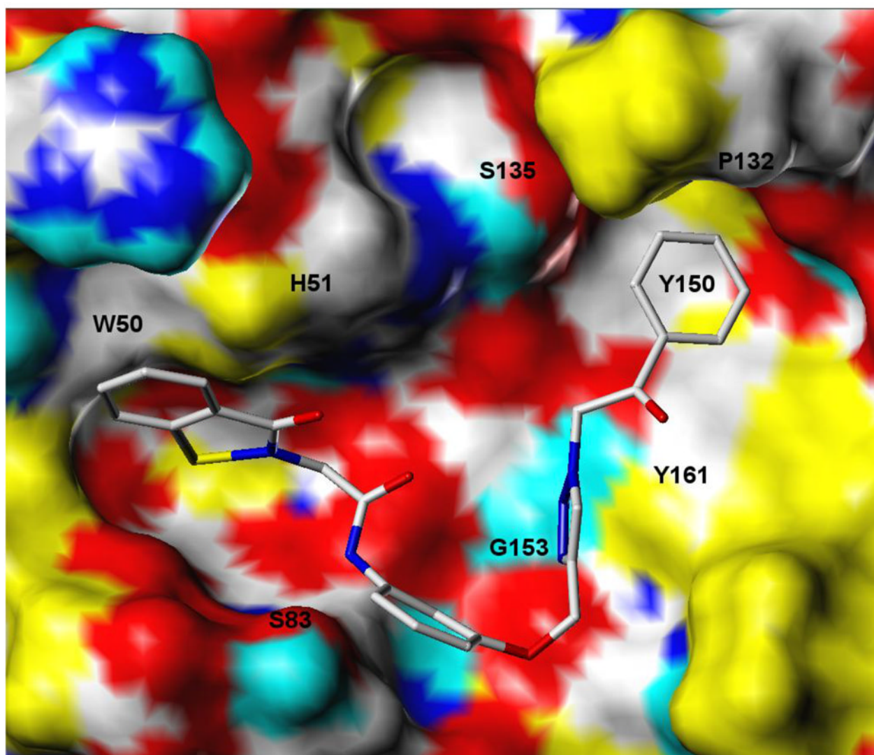
Figure 7. Conformation for inhibitor 7j bound to the catalytic site of DENV2 NS2B-NS3 protease, as predicted from molecular docking simulations. The receptor surface is colored as follows: red = polar O, blue = polar N, cyan = polar (donatable) H, white = weakly polar aliphatic or aryl CH groups, yellow = nonpolar lipophiles. The ligand is rendered in stick form according to standard CPK coloring.
