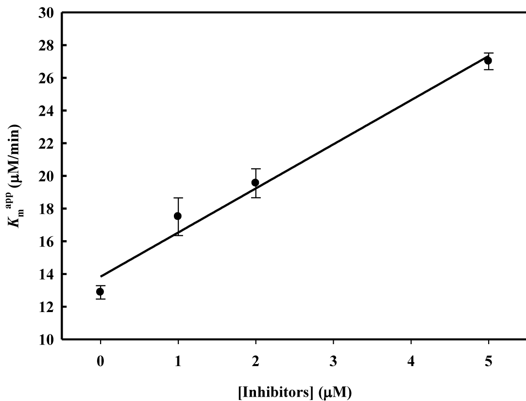
Figure 6. Plot of K_m values versus concentration of compound 7n . K_m values with no inhibitor and at different concentrations of inhibitor were calculated and plotted versus different concentrations of inhibitor. From these data, the Slope = 2.6988 \pm 0.2712 \mu\text{M} and the Intercept = 12.8732 \pm 0.7427 \mu\text{M} were obtained and the K_i value calculated from the equation Intercept / Slope is 4.77 \pm 0.05 \mu\text{M} .
