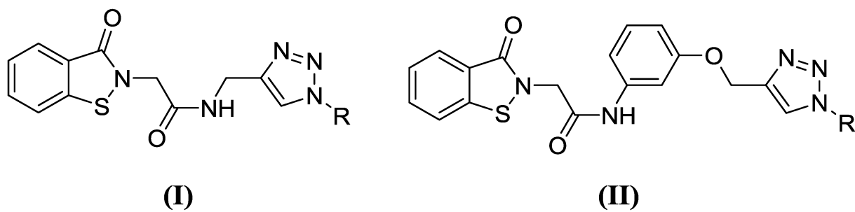
Figure 1. General structures of DENV2 NS2B-NS3pro inhibitors (I-II).
