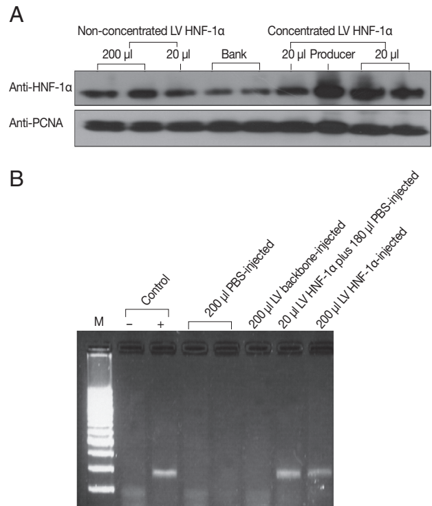
Fig. 1. Expression of LV HNF-1 \alpha . (A) Western blot using an anti-HNF-1 \alpha antibody in HeLa cells transfected with concentrated or non-concentrated LV HNF-1 \alpha and using an anti-PCNA antibody as a loading control. (B) HNF-1 \alpha mRNA expression in transduced mice liver tissues as assessed by RT-PCR.
