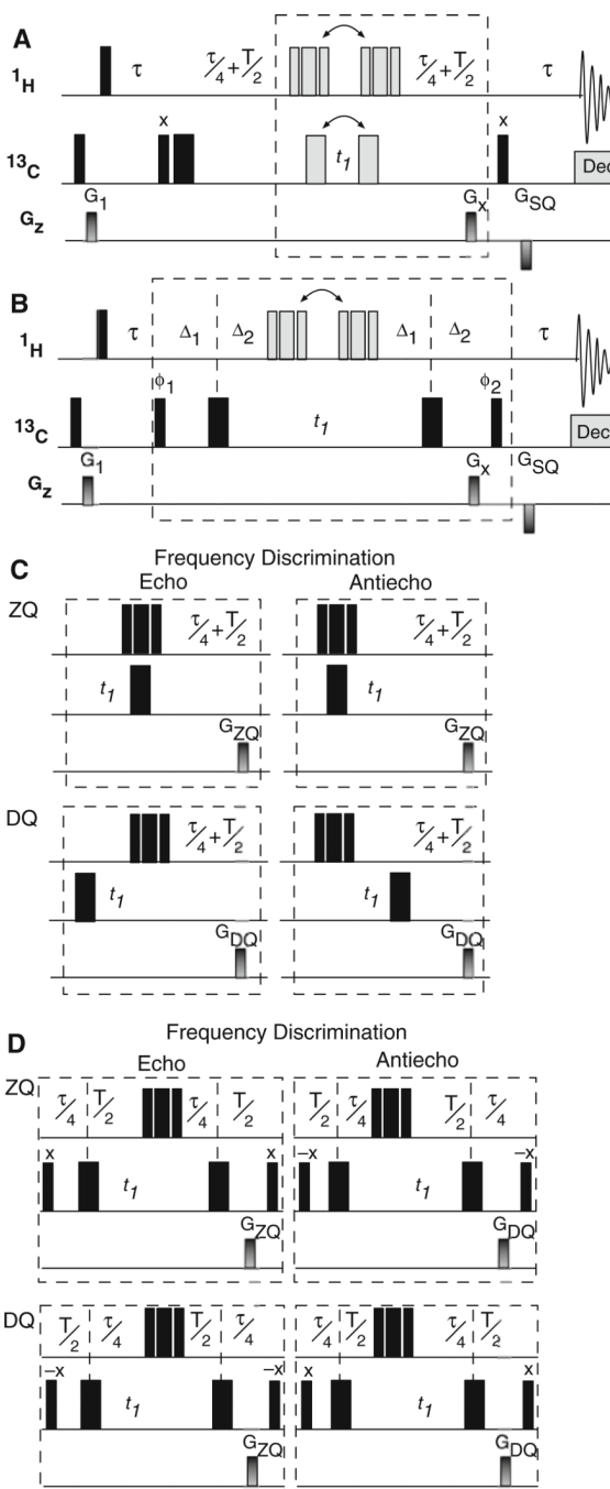
Fig. 3. Hahn-echo gsHZQC pulse sequences for measurement of multiple-quantum transverse relaxation rates. a In the first half of the methyl multiplet filter, ZQ or DQ coherence is selected during the relaxation period ( T ) using a pulse sequence element shown in part C and similar to Fig. 2. b In the second half of the multiplet filter, the phase of the outer multiplet components is inverted using a pulse sequence element shown in part D. c A grid similar to that in Fig. 2 describes the evolution of magnetization through the pulse sequence in (a). In this case, the rows correspond to the multiple quantum coherence (ZQ or DQ) present during the relaxation delay and only one phase of the outer multiplet components is considered. The coherence selection (ZQ or DQ) during the relaxation delay is controlled by
