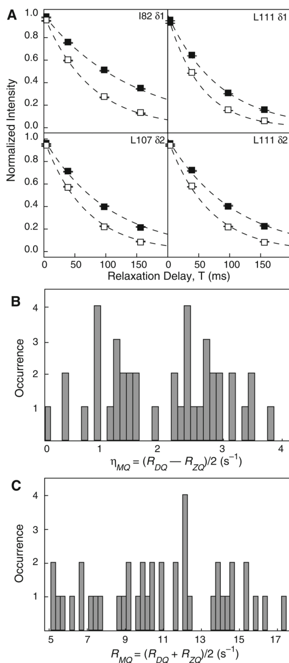
Fig. 5. Measurement of multiple-quantum transverse relaxation rates in RNase H. a Zero- and double-quantum relaxation profiles, R_{ZQ} (filled squares) and R_{DQ} (open squares), are shown for selected residues. Dashed lines are the best fits of a monoexponential decay to the respective profiles. Peak intensities were normalized and averaged for display. Error bars are smaller than the plotted symbols and represent the error associated with the averaged data sets. The mean \pm one standard deviation of R_{DQ} and R_{ZQ} for two data sets are 13.3 \pm 0.1 \text{ s}^{-1} and 6.9 \pm 0.1 \text{ s}^{-1} for I82 \delta 1 , 19.9 \pm 0.1 \text{ s}^{-1} and 13.0 \pm 0.2 \text{ s}^{-1} for L107 \delta 1 , 17.7 \pm 0.4 \text{ s}^{-1} and 13.0 \pm 0.2 \text{ s}^{-1} for L111 \delta 1 , and 18.9 \pm 0.2 \text{ s}^{-1} and 12.0 \pm 0.1 \text{ s}^{-1} for L111 \delta 2 , respectively. b and c Histograms of \eta_{MQ} = (R_{DQ} - R_{ZQ})/2 and R_{MQ} = (R_{DQ} + R_{ZQ})/2 for
