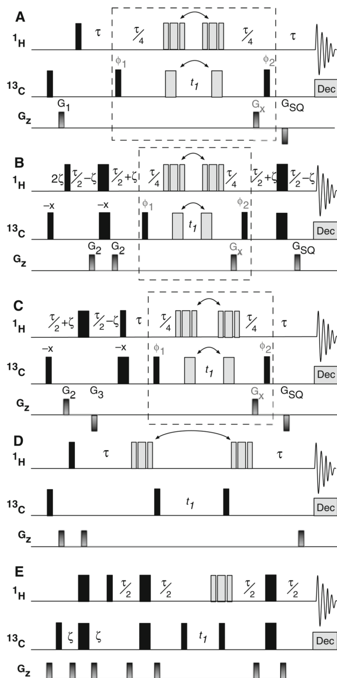
Fig. 1. Comparison of gradient selected pulse sequences for measuring ^1\text{H} - ^{13}\text{C} heteronuclear zero-quantum coherences (gsHZQC) to previously proposed HZQC schemes (Tugarinov et al. 2004; Ollerenshaw et al. 2005). a A simple implementation of the gsHZQC experiment. The dashed box denotes four distinct parts of the pulse sequence: two for inversion of the outer multiplet components and two for echo/antiecho frequency discrimination during t_1 . These alterations are achieved by a pulse sequence element in which the positions of the composite ^1\text{H} ( 90_x-180_y-90_x ) and 180^\circ ^{13}\text{C} pulses flanking t_1 (gray bars) are shifted (see Fig. 2). The phases \phi_1 and \phi_2 are given in Fig. 2 for the first step of the phase cycle. The 90^\circ ^{13}\text{C} pulse labeled \phi_1 and the receiver are inverted on alternate scans for isotope
