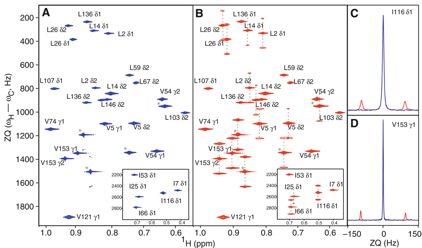
Fig. 4. Comparison of gsHZQC and unfiltered HZQC pulse sequences. a A gsHZQC (Fig. 1a) spectrum of selected Leu \delta 1 and \delta 2 and Val \gamma 1 and \gamma 2 resonances in the methyl region of RNase H. A region containing Ile \delta 1 resonances are shown in the inset . Unassigned peaks are marked with an asterisk . b An unfiltered HZQC (Fig. 1d, Tugarinov et al. 2004) spectrum of the same region. Dashed lines connect the outer multiplet components to the central component. Both (a) and (b) were collected at 21.1 T and contour levels have been normalized to their respective noise floors. c and d Comparison of traces along the t_1 dimension of HZQC pulse sequences for I116 \delta 1 ( c ) and V153 \gamma 1 ( d ). Colors are as in (a) and (b)
