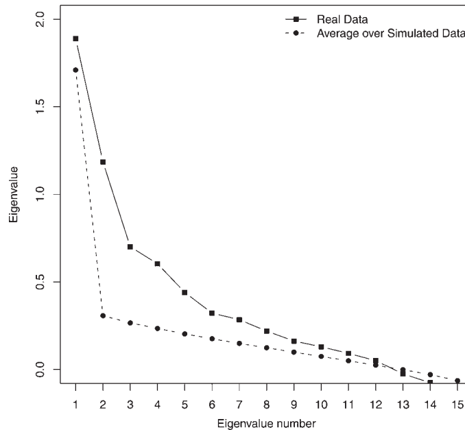
Fig. 2. Scree plot depicting the results of the modified parallel analysis for the 15-item list. The real data (solid line) show evidence of a two-factor solution based on the second eigenvalue >1.0 and the difference between the second eigenvalues of the real data the simulated data (dashed line).
