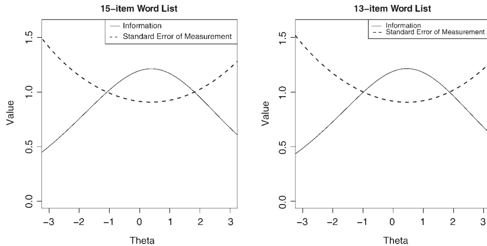
Fig. 4. Test information and standard error of measurement for the 15-item (left) and 13-item (right) 2PL IRT models. The similarity between the curves suggests that the measurement properties of the 15-item model are not impacted by the removal of the final two items.
