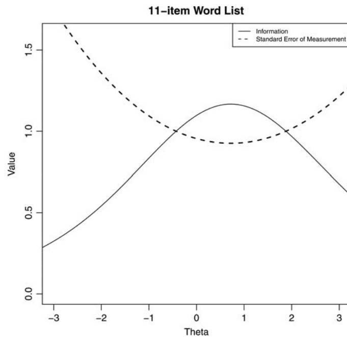
Fig. 6. Test information and standard error of measurement for the 11-item 2PL IRT model.
