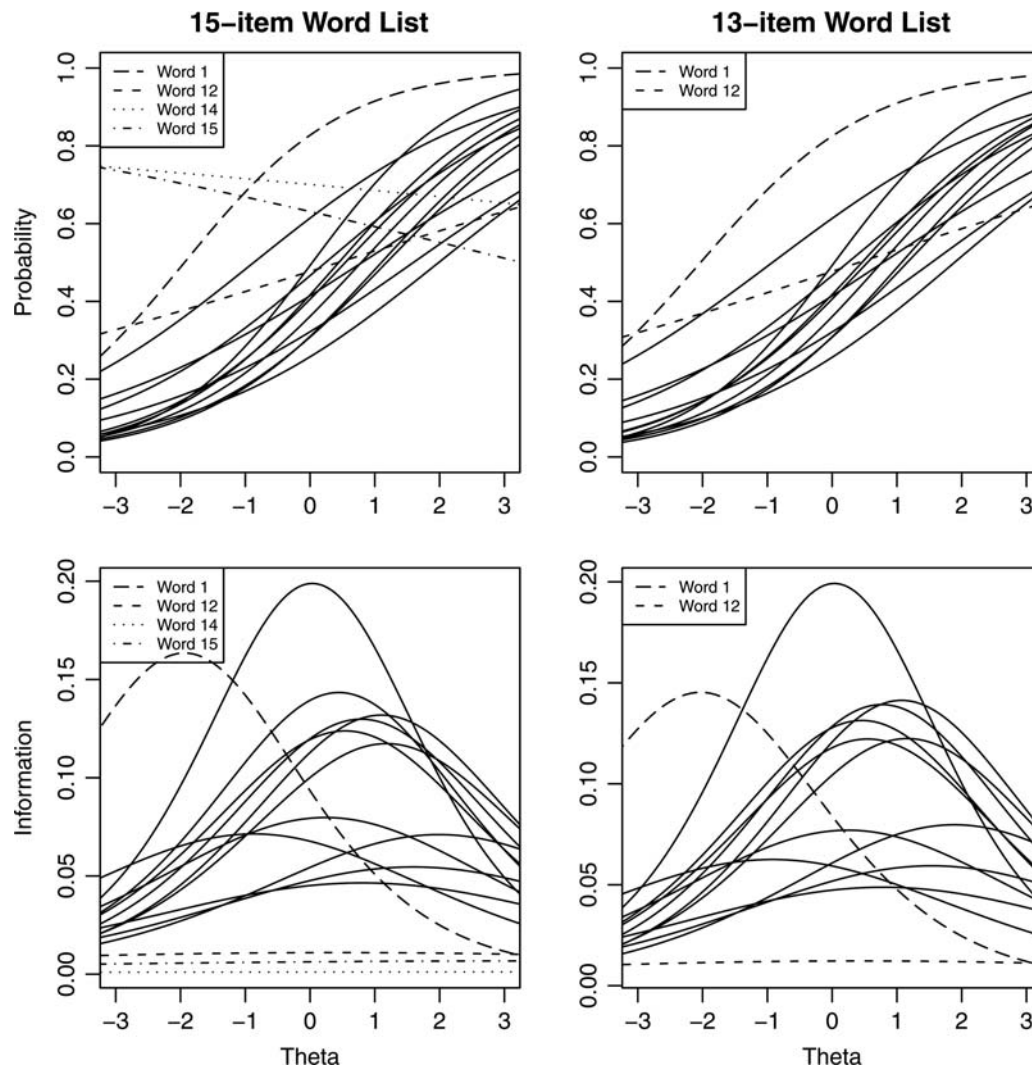
Fig. 3. Item characteristic (top row) and item information (bottom row) curves for the 15-item (left column) and 13-item (right column) 2PL IRT models. In the 15-item model, items 1, 12, 14, and 15 (broken lines) function dissimilarly from the remaining items (solid lines). Removing items 14 and 15 to yield a 13-item list did not improve the fit of items 1 and 12.
