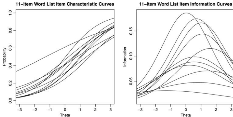
Fig. 5. Item characteristic (left) and item information (right) curves for the 11-item 2PL IRT model.
