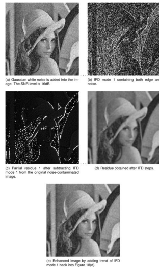
Figure 18. Edge restoration/compensation and edge enhancement using edge-noise-decoupling technique based on IFD mode reconstruction.
