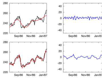
Figure 8. IFD analysis for the half-year S&P500 index centered on Oct 19, 1986, one year before Black Monday crash. The panels and notations are same as those in Figure 7. The magnitude of the oscillations of various modes are much smaller than those in the year of big crash.
