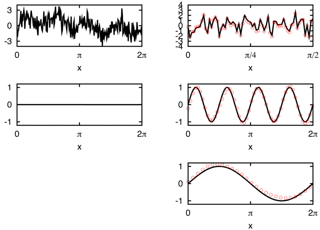
Figure 4. IFD analysis for signal \sin(x) + \sin(4x) + \text{noise} . The signal-to-noise ratio (SNR) is -6\text{dB} . The panel on the top left shows the original signal. The three panels on the right show IFD modes 1 (which is high frequency noise), 2 (i.e. \sin(4x) ) and 3 ( \sin(x) ) respectively. Black solid curves show the exact values, and red circles show the IFD results. The bottom left one shows the residue after the above 3 modes are subtracted from the original signal.
