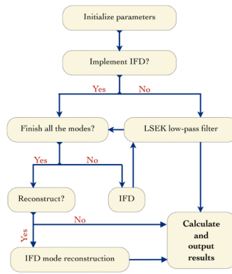
Figure 1. Chart sketch summarizing the LSEK based IFD.
