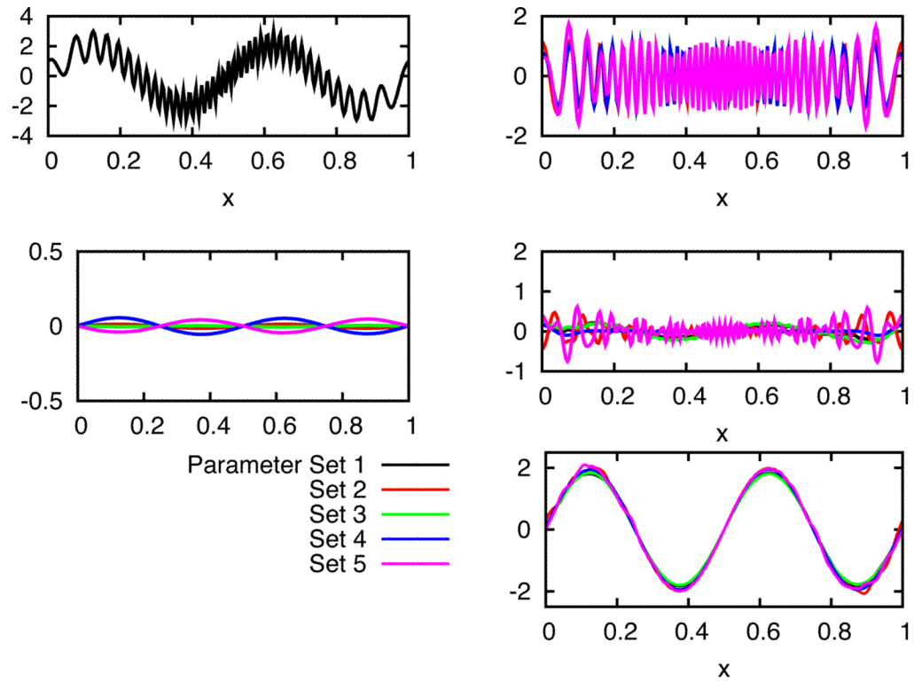
Figure 5. IFD analysis for signal \cos(4\pi\lambda(x) * x) + 2 \sin(4\pi x) . The panel on the top left shows the original signal. The three panels on the right show IFD modes 1 (which is high frequency noise), 2, and 3, respectively. The bottom left one shows the residue after the above 3 modes are subtracted from the original signal. In each individual panel, there are 5 lines embedded and closely overlapping with each other, corresponding to the various choices of parameters listed in Table 1.
