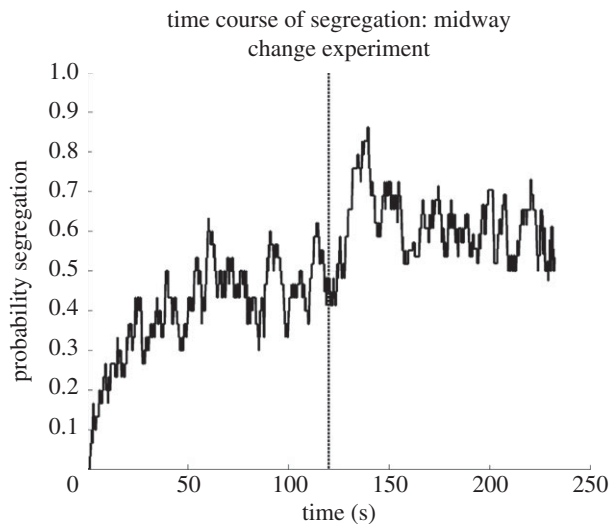
Figure 2. Time course of the probability of reporting segregation throughout a 4-min ‘ABA 2 ’ sequence with 150-ms stimulus onset asynchrony between consecutive tones. At 120 s (marked by the bold dashed line on the figure), the frequency difference between the ‘A’ and ‘B’ sets of tones is suddenly increased from five to seven semitones. Note that no perceptual reset towards the integrated organization is reported by participants.
