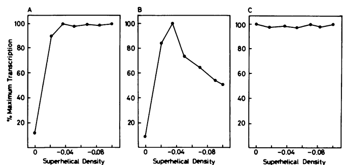
Figure 3. In vitro transcription from templates of varying superhelical density. A, transcription of the fibroin gene on pFb205 DNA. B, transcription from the Ad2 MLP on pML(C 2 AT) DNA. C, transcription of the hsp70 gene on p56H8RIA DNA. Each topoisomer preparation was tested for transcription activity as described under 'MATERIALS AND METHODS'. The activity was expressed as percentage of the maximal value for transcript of each gene and plotted versus superhelical density of the DNA template. The maximal values were 3,800cpm in A, 5,900cpm in B, and 5,400cpm in C.
