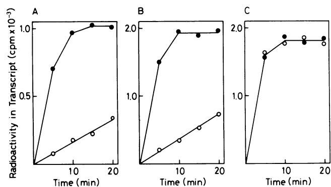
Figure 4. Time required for the assembly of preinitiation complex. A , relaxed closed circular DNA (○) or supercoiled plasmid DNA ( \sigma = -0.06 ) of pFb205 (●) was preincubated for the indicated times and preinitiation complexes formed were assayed as described under 'MATERIALS AND METHODS'. B , same as in A except that relaxed closed circular DNA (○) or partially superhelical DNA ( \sigma = -0.036 ) of pML(C 2 AT) (●) was used as the template. C , same as in A except that relaxed closed circular DNA (○) or supercoiled plasmid DNA ( \sigma = -0.06 ) of p56H8RIA (●) was used as the template.
