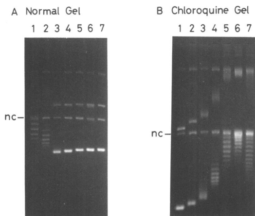
Figure 2. Agarose gel electrophoresis of DNA topoisomers. Portions (125ng in A and 250ng in B) of each topoisomer population of pML(C 2 AT) DNA were electrophoresed in a 1% agarose gel with (B) or without (A) 15 \mu\text{g}/\text{ml} of chloroquine as described under 'MATERIALS AND METHODS'. Lane 1, \sigma = 0 ; Lane 2, \sigma = -0.021 ; Lane 3, \sigma = -0.036 ; Lane 4, \sigma = -0.051 ; Lane 5, \sigma = -0.071 ; Lane 6, \sigma = -0.091 ; Lane 7, \sigma = -0.100 . In this chloroquine gel, topoisomers in lanes 1 to 5 are migrating as positively supercoiled DNA whereas those in lane 7 are migrating as negatively supercoiled DNA as determined by comparison with other gel containing less chloroquine. nc represents the position of nicked circular DNA.
