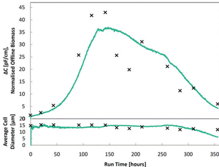
Figure 1 Online and offline measurements of a CHO cell culture process. Top : online capacitance (solid line) and normalised ViCell biomass volume (crosses). Bottom : estimated average cell diameter from online capacitance (solid line) and ViCell system (crosses).
