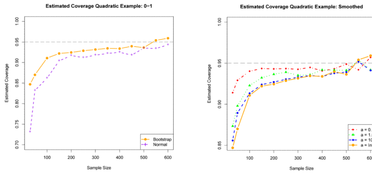
Figure 1. Left: Coverage of centered percentile bootstrap and normal approximations for constructing confidence sets for \tau(\hat{c}) . Right: Coverage of centered percentile bootstrap with smoothed target \tau_{smoothed}(\hat{c}) \triangleq P(1 + \exp(aY\hat{c}(X)))^{-1} for varying values of a ; a value of a = \infty corresponds to \tau(\hat{c}) . Results are based on 1000 Monte Carlo iterations, target coverage is .950. The performance of the ACI on this example can be found in Section 5 under the example labeled “quad.”
