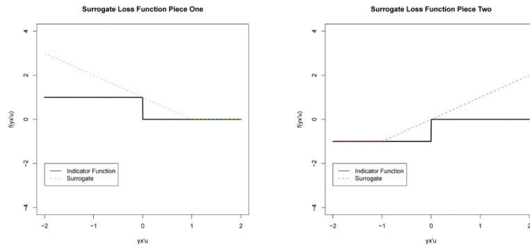
Figure 2. Relaxation of the indicator functions. Left panel: indicator function 1_{yx^t u < 0} replaced with convex surrogate (1 - yx^t u)_+ . Right panel: indicator function -1_{yx^t u < 0} replaced with convex surrogate (1 + yx^t u)_+ - 1 .
