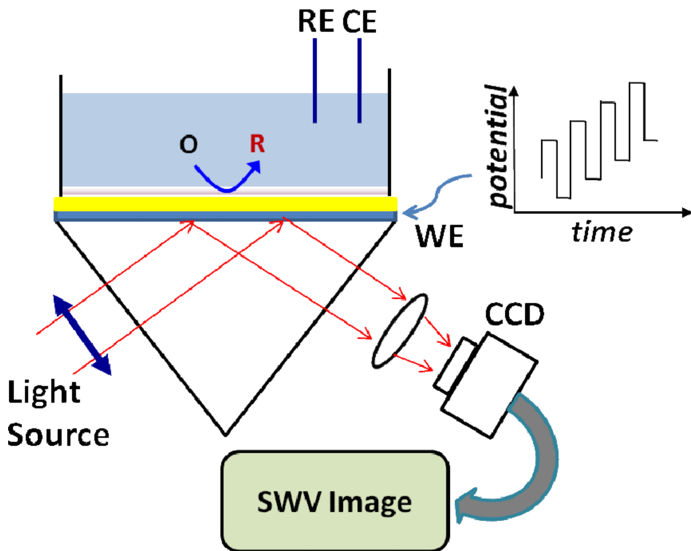
Scheme 1. Experiment setup of SWV imaging. See text for details.
