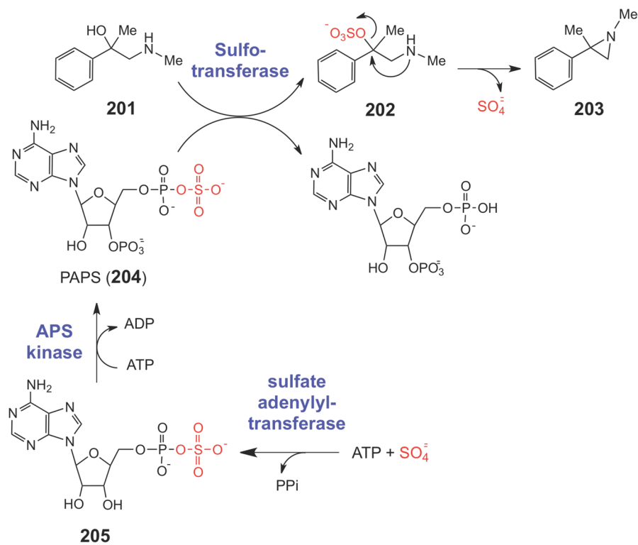
Scheme 35.
