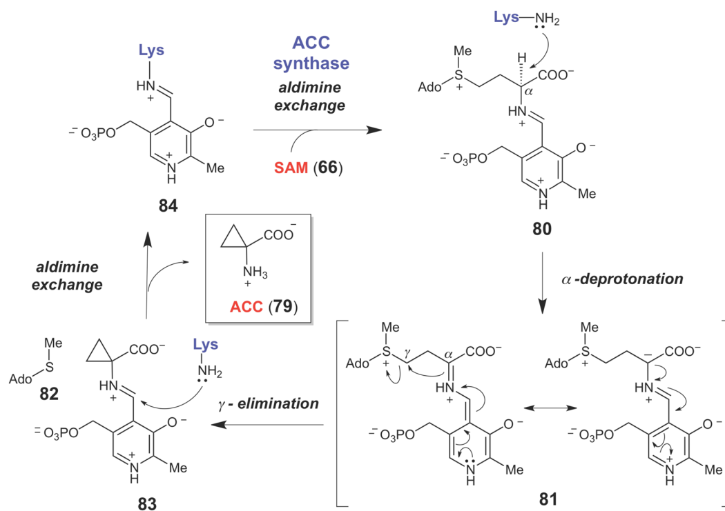
Scheme 12.
