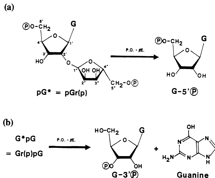
Fig. 4. Summarized results of periodate oxidation followed by \beta -elimination (P.O. - \beta E.) procedure applied: (a) to pGr(p) mononucleotide: identification of guanosine-5'-phosphate (G-5'P) as oxidative compound, (b) to Gr(p)pG dinucleotide: identification of guanosine-3'-phosphate (G-3'P) and guanine as oxidative products.
