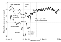
Figure 4. Correcting the ladder for context effects
