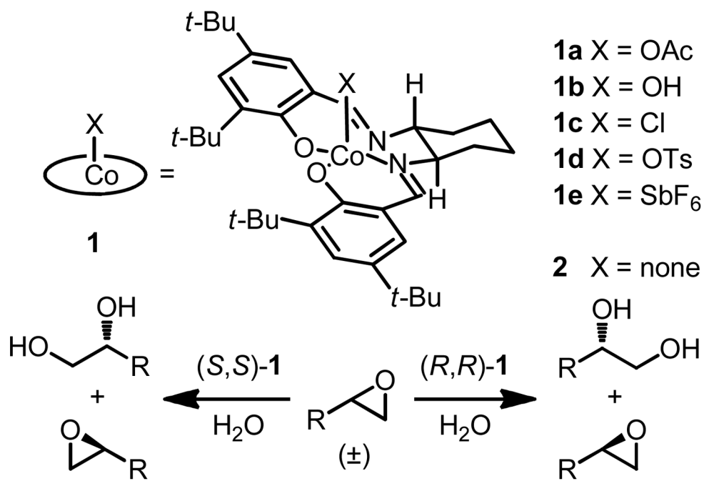
Scheme 1. Hydrolytic kinetic resolution of terminal epoxides catalyzed by (salen)Co(III) complexes
