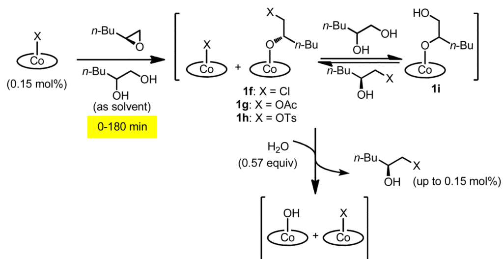
Scheme 3. Delayed-addition of water to probe catalyst partitioning.
