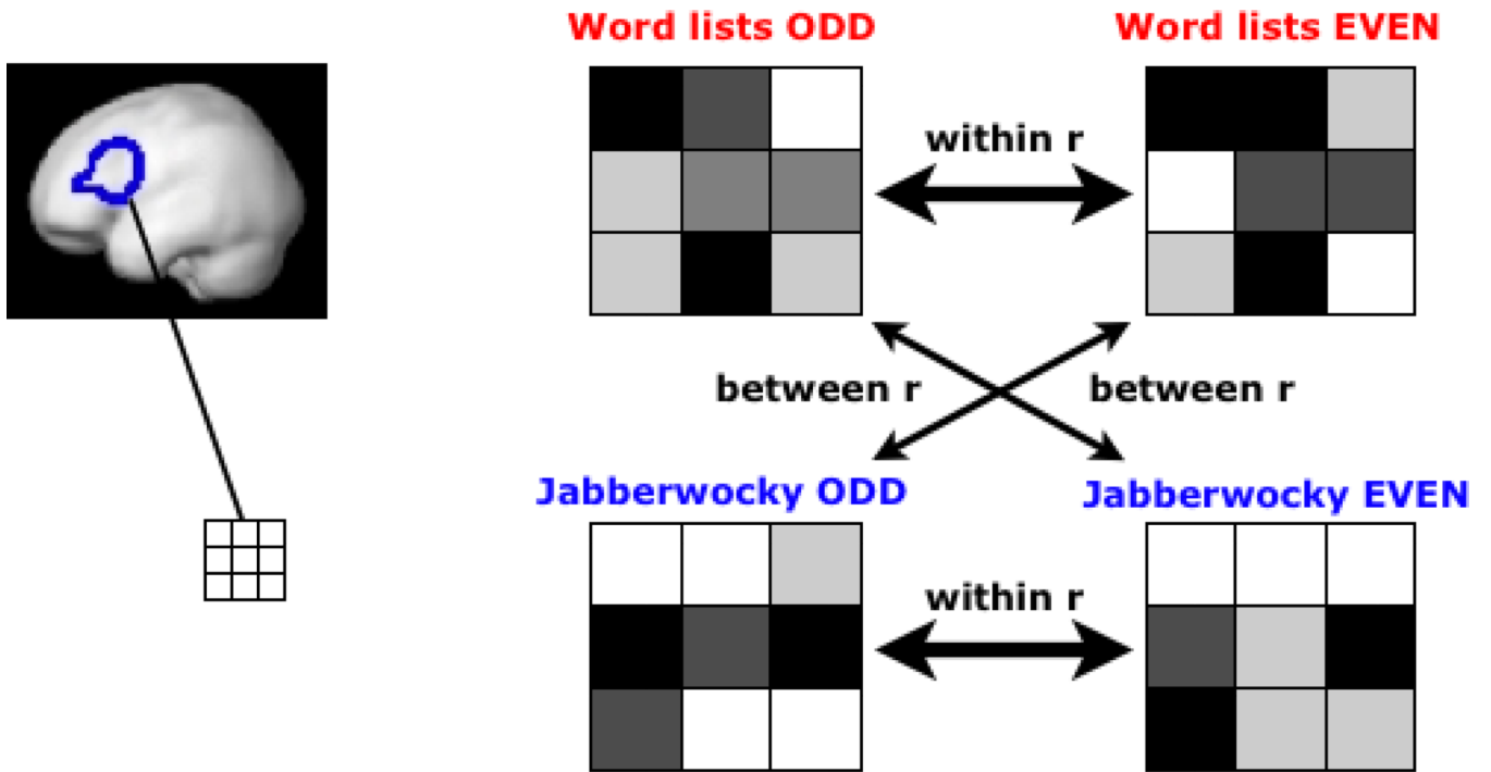
Figure 4. (adapted from a figure by Julie Golomb): A schematic illustration of the logic of the correlation-style multi-voxel pattern analyses (Haxby et al., 2001).
