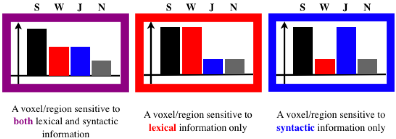
Figure 2. Idealized functional profiles of response for a voxel or a region that is sensitive to both lexical and syntactic information (purple frame), to lexical information only (red frame), and to syntactic information only (blue frame). S=sentences, W=Word-lists, J=Jabberwocky sentences, N=Nonword lists.
