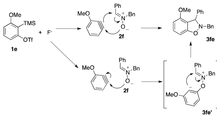
Scheme 1. Possible Mechanisms
