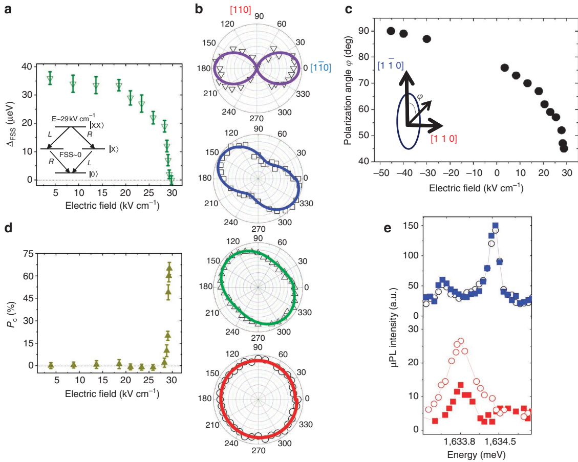
Figure 2 | Electric field-dependence of fine-structure splitting energy and QD exciton polarization. (a) Variation of \Delta_{\text{FSS}} (closed-down triangles) with the electric field. The inset shows a sketch of the biexciton–exciton cascaded emission for E=29\text{ kV cm}^{-1} ( \Delta_{\text{FSS}}=0 ). (b) Linear polarization dependence of the exciton X at various electric fields (from top): E = -45, 22, 27 and 29.2\text{ kV cm}^{-1} , relative to [1\bar{1}0] , the sample’s crystallographic axis. All polar plots have an axis scale increment of 10\text{ }\mu\text{eV} . The solid lines represent a fit to the data with a sinusoidal function. (c) Variation of the exciton polarization angle \varphi with the electric field. The inset describes the angle \varphi relative to the crystal axis [1\bar{1}0] . The exciton PL emission cannot be seen when -30 < E < -0.2\text{ kV cm}^{-1} . (d) Evolution of the degree of exciton PL circular polarization P_c (closed-up triangles) with the electric field. (e) Circular polarization resolved detection \sigma^+ (open-circles) and \sigma^- (closed-squares) of the exciton PL spectra at two different electric fields: 23\text{ kV cm}^{-1} (top) and 29.2\text{ kV cm}^{-1} (bottom).
