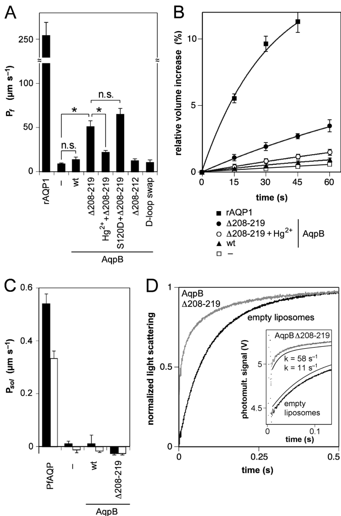
FIGURE 3. Functional analysis of AqpB wild-type and mutants. A, the water permeability of AqpB wild-type and mutants in comparison to rat AQP1 ( rAQP1 ) expressing X. laevis oocytes and to buffer-injected oocytes (-). The AqpB \Delta 208-219 mutant was further inhibited by 300 \mu\text{M} \text{Hg}^{2+} . The bars indicate the permeability coefficient ( P_f ) derived from swelling rates in a 140 mosm/kg inward-directed osmotic gradient. The error bars denote the S.E. from 7–10 experiments. *, significantly different P_f values, p < 0.01 . n.s., non-significant difference. B, the original oocyte swelling curves used for the calculation of the P_f values are shown. The data points ( \pm S.E.) are connected by single exponentially fitted curves. C, glycerol (filled bars) and urea (open bars) permeability coefficients ( P_{sol} ) are plotted as obtained from X. laevis oocyte swelling in a 130 mM isotonic chemical gradient. The aquaglyceroporin from P. falciparum ( PfAQP ) and buffer-injected oocytes (-) served as controls ( n = 7-10 ). D, water permeability of AqpB \Delta 208-219 was confirmed by stopped-flow light scattering with proteoliposomes and empty liposomes in an outward osmotic gradient of 200 mosm/kg. Nine traces were averaged and normalized for each experiment. Reconstitution and assays were repeated twice with equal results. The inset depicts the original, non-normalized photomultiplier readings for the first 110 ms. Signal artifacts are seen within the 10-ms dead time. The curves derived from single exponential fits (smooth lines) and respective rate constants ( k ) are plotted next to the raw data.
