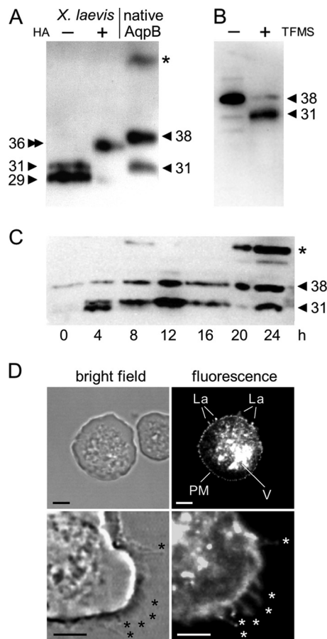
FIGURE 4. Expression, glycosylation, and localization of AqpB in D. discoideum . A, the Western blot analysis using an anti-AqpB antiserum shows native AqpB in comparison to AqpB heterologously expressed in X. laevis oocytes with and without an N-terminal HA tag. The apparent molecular masses are indicated (kDa). A 90-kDa band labeled with an asterisk is not specific. B, trifluoromethanesulfonic acid (TFMS) was used for chemical deglycosylation of native AqpB. The shift in molecular weight from 38 kDa to 31 kDa is shown by Western blot analysis. C, the Western blot shows AqpB expression levels during a full developmental cycle of D. discoideum over 24 h. Both glycosylated (38 kDa) as well as non-glycosylated AqpB (31 kDa) is seen. An additional smaller band in the 4 h lane corresponds to translation from Met-18 of AqpB. A nonspecific 90-kDa band is labeled with an asterisk. D, AqpB was localized in D. discoideum amoebae by expression of a C-terminal GFP-fusion construct. The upper panel (scale bar = 5 \mu\text{m} ) shows a bright field image of one transformed (left panel) and one untransformed amoeba (right panel). In the GFP excitation channel, only the transformed amoeba exhibit fluorescence. Lamellipodia-like protrusions (La) of the plasma membrane (PM) and intracellular vacuolar structures (V) are labeled in the upper panel. The lower panel shows a higher magnification view for visualization of the plasma membrane protrusions (asterisks).
