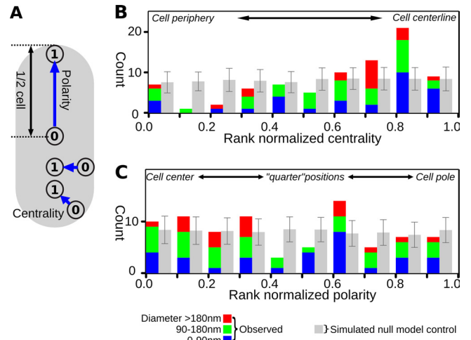
FIG 4 Granule localization is biased toward the central region of the cell. (A) Cartoon to illustrate the centrality and polarity metrics. (B) Distribution of rank-normalized centrality of observed granules (colored bars) and a data set randomized 100 times (gray bars; error bars are standard deviation across all 100 randomizations to illustrate the significance of the deviation of observed granules from the null model). Note that granules occur around the cell periphery less than would be expected at random and more toward the center than would be expected. (C) Polarity of granules as a function of size across the first three time points, alongside mean and standard deviations of 100 further randomizations of the observed data set (gray).
