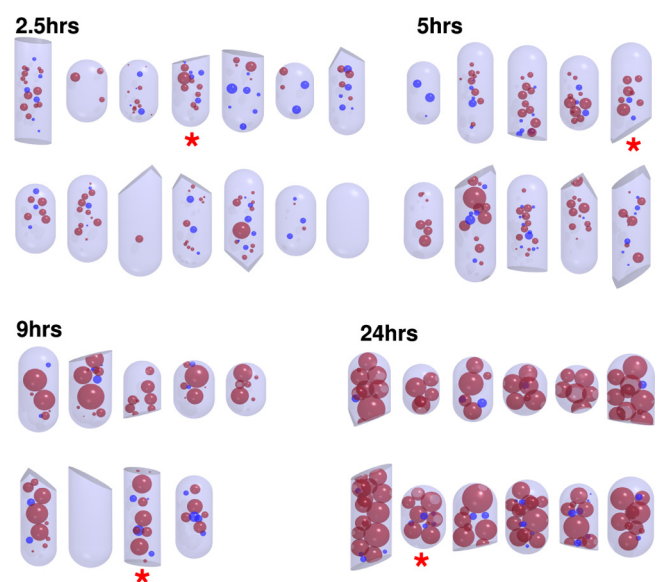
FIG 2 Quantitative models. 3-D models of all 45 cells. Asterisks mark models of the cells depicted in Fig. 1. Red granules represent PHB; blue indicates polyphosphate.
