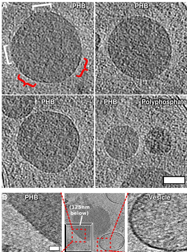
FIG 3 Surface features of granules. (A) Computational slices through representative medium-sized PHB granules (top and bottom left) and, for comparison, PHB immediately to the left of a polyphosphate granule (bottom right) to illustrate difference in surface structure and density. Red curly brackets (top left) highlight the presence of a discernible, patchy surface layer; white square brackets the absence. Bar, 100 nm. (B) Slices (12.6 nm thick) through a granule isolated from a lysed cell (middle; “drop-away” inset at bottom left depicts another Z-slice through the tomogram so as to depict the optimal cross section through PHB granule, 125 nm beneath the main slice with an optimal cross section through vesicle). Close-ups of PHB surface (left) and vesicle membrane (right) demonstrate by direct comparison the lack of membrane on the granule surface. Note that the close-up of the granule is of the area with most pronounced surface. Bar, 50 nm. Scales of PHB and vesicle close-up panels are the same.
