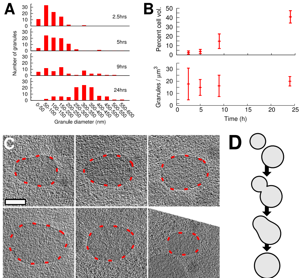
FIG 5 Granules are constantly being initiated and progressively fuse. (A) Distribution of granule sizes in cells from the four time points showing constant presence of small (<100-nm) granules. Note that cells at later time points are thicker, meaning that we may not have been able to detect the smallest granules in these cells. (B) Overall granule volume increases with time (top), and the number of granules per unit volume remains roughly constant over all time points (bottom). (C) Examples of nonspherical granules as candidates for fusion processes. Granules have been rotated so that the long axis of the nonspherical granules is horizontal in the plane of the figure; areas of indistinct detail are thus a result of the “missing wedge” of data in reciprocal space inherent to ECT. (D) Model of the time course of granule fusion. Granules depicted in C are caught at the third stage of fusion.
