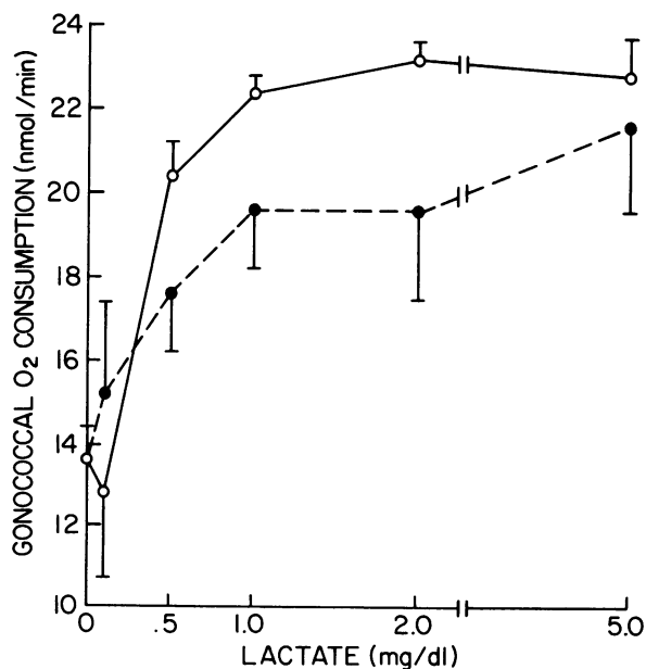
Figure 5. Dose-response curves of the effect of L(+) (—) and D(-) (---) isomers of lactic acid on the maximal O 2 consumption rate of gonococci ( 10^9 /ml) suspended in HBSS ( n = 3 ).
