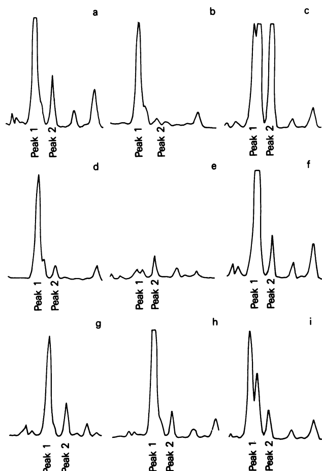
Figure 2. Determination of chemical structure of methionine oxidation product in the urine of MAT-deficient patient. (a) Portion of amino acidogram of patient's untreated urine (40 μl). Peak 1 contains unknown compound and threonine. Peak 2 represents serine. (b) After periodate treatment. Threonine is gone from peak 1; serine from peak 2. (c) Same as a, but with added serine and threonine. (d) Same as c, after periodate treatment. (e) Same as a, after 2-mercaptoethanol treatment. Peak 1, containing unknown compound, is diminished. (f) Same as a, but with added methionine sulfone, which elutes with peak 1. (g) Same as f, after 2-mercaptoethanol treatment. Methionine sulfone is relatively insensitive to 2-mercaptoethanol. (h) Same as a, but with added L-methionine- d -sulfoxide. Note single peak. (i) Same as a, but with added L-methionine- l -sulfoxide. Two peaks indicate that unknown compound is not the L-l -diastereoisomer.
