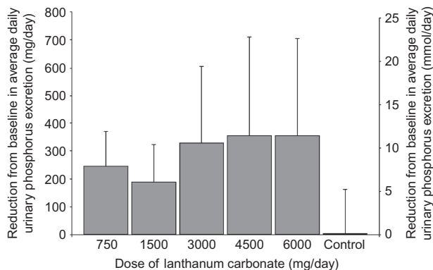
Figure 1. Mean ± SD reduction from baseline in average daily urinary phosphorus excretion at different doses of lanthanum carbonate (study 1).
