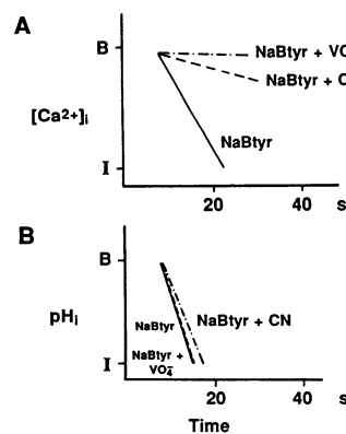
Figure 6. Effects of cyanide and vanadate inhibitors on the initial rate of butyric acid stimulated Ca 2+ efflux and acidification. Vanadate and cyanide inhibited the reduction of [Ca 2+ ] i stimulated by NaBtyr but did not affect the change in pH i produced by the metabolic acid. Data are the mean of the initial rates of five experiments.
