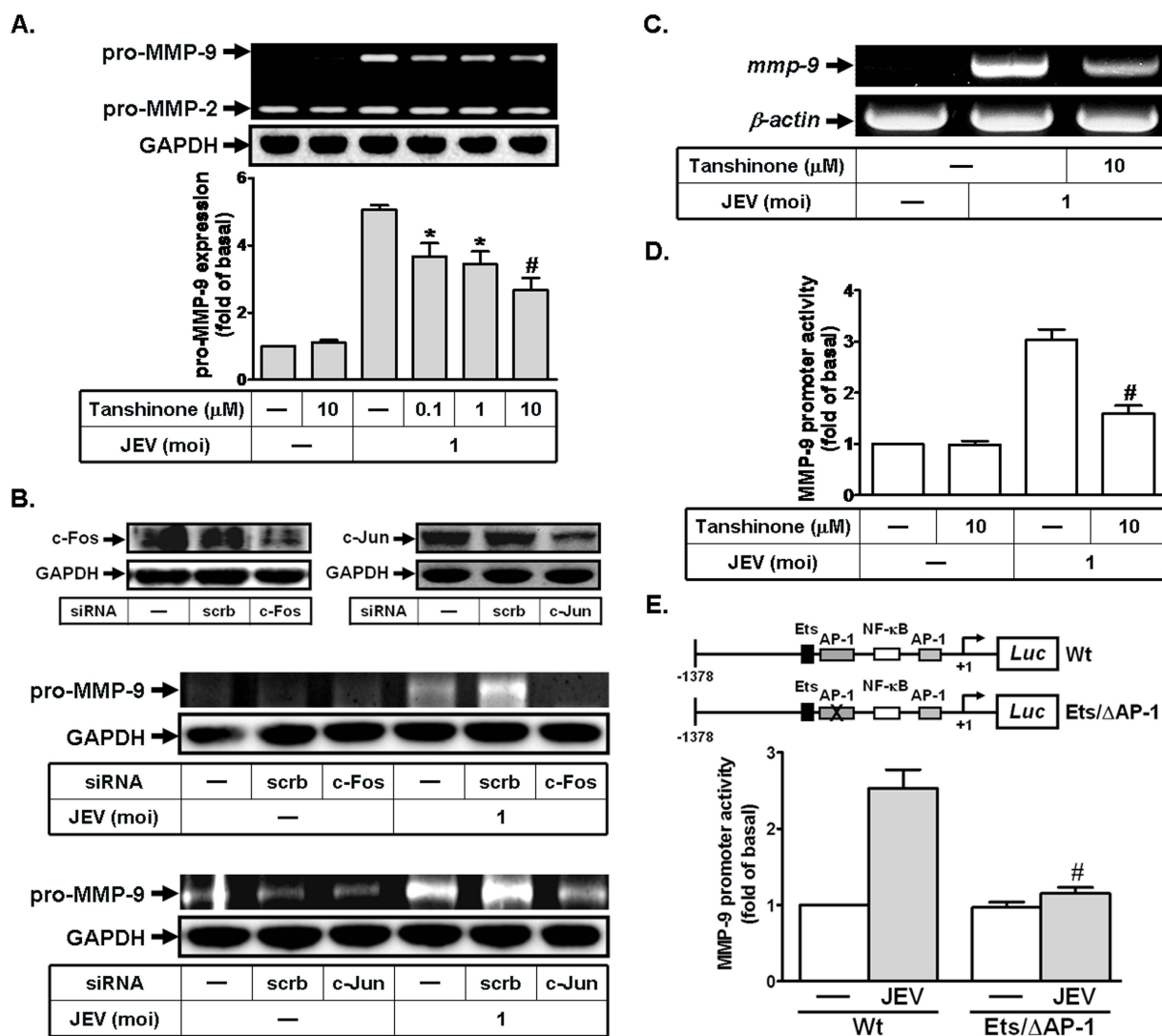
Figure 1 Involvement of AP-1 in MMP-9 expression with JEV infection of RBA cells. (A, B) Cells were pretreated with tanshinone for 1 h or transfected with siRNA of scrambled (scrub), c-Jun, or c-Fos, and then infected with JEV for 16 h. The conditioned media were used to determine MMP-9 expression by gelatin zymography. Cell lysates were analyzed by western blot using an anti-c-Jun, anti-c-Fos, or anti-GAPDH antibody. (C) Cells were pretreated with tanshinone for 1 h, and then incubated with JEV for 6 h. RNA samples were analyzed by RT-PCR to assess the levels of MMP-9 mRNA expression. (D, E) Cells were transiently transfected with MMP-9-luc reporter gene, pretreated with tanshinone (10 μM) for 1 h, and then incubated with JEV for 6 h. In addition, cells were transfected with wild-type MMP-9 promoter and AP-1-mutated MMP-9 promoter, and then incubated with JEV (moi = 1) for 6 h. MMP-9 promoter activity was determined in the cell lysates. Data are expressed as mean ± S.E.M. for five independent experiments. *P < 0.05; #P < 0.01, as compared with the cells exposed to JEV alone (A, D). #P < 0.01, as compared with cells transfected with wild-type MMP-9 promoter stimulated by JEV (E).
