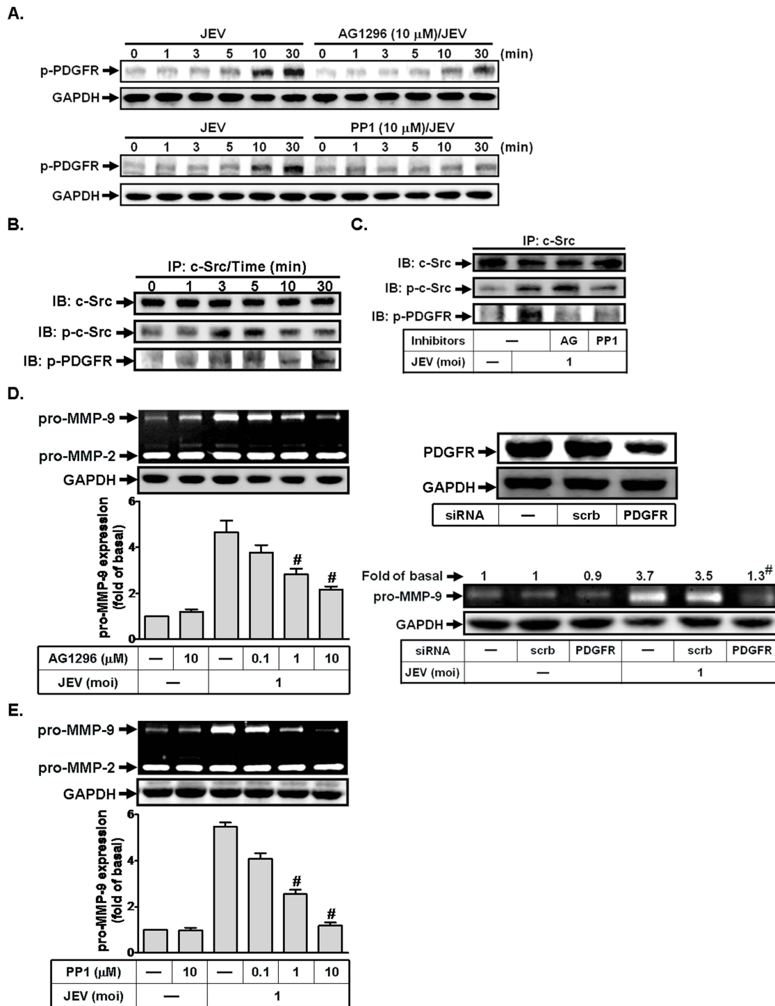
Figure 3 JEV infection induces MMP-9 expression through c-Src/PDGFR in RBA-1 cells. (A) Cells were pretreated with AG1296 (10 \mu\text{M} ) or PP1 (10 \mu\text{M} ) for 1 h, and then infected with JEV (moi = 1) for the indicated time intervals. The cell lysates were analyzed by western blot using an anti-phospho-PDGFR or anti-GAPDH antibody. (B, C) Cells were pretreated without or with AG1296 (AG, 10 \mu\text{M} ) or PP1 (10 \mu\text{M} ) for 1 h, and then incubated with JEV (moi = 1) for the indicated time intervals (B) or 5 min (C). Cell lysates were subjected to immunoprecipitation using an anti-c-Src antibody. The immunoprecipitates were analyzed by western blot using an anti-c-Src, anti-phospho-c-Src, or anti-phospho-PDGFR antibody. (D, E) Cells were pretreated with AG1296 or PP1 for 1 h or transfected with PDGFR siRNA, followed by incubation with JEV for 16 h. Cell lysates were analyzed by western blot using an anti-PDGFR or anti-GAPDH antibody. The conditioned media were used to determine MMP-9 expression by gelatin zymography. Data are expressed as mean \pm S.E.M. for five independent experiments. ^{\#}P < 0.01 , as compared with cells exposed to JEV alone [D (left panel), E]. ^{\#}P < 0.01 , as compared with cells transfected with scrambled siRNA exposed to JEV (D, right panel).
